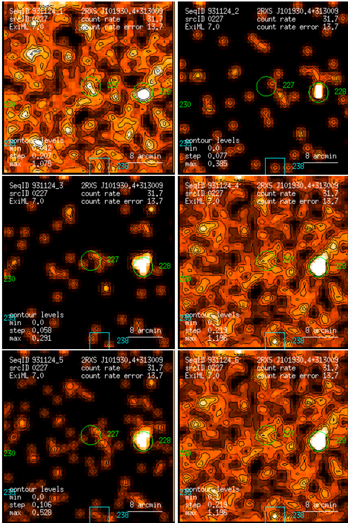
Figure 227: RASS 931124: detection 0227: band rate images, Gaussian filter: (1) PSPC channels 11 – 41, (2) 52 – 90, (3) 91 – 201, (4) 11 – 235, (5) 52 – 201, (6) 11 – 201. Broad band rates in counts/ks. Band rate contour levels in counts/ks/arcmin 2 .
