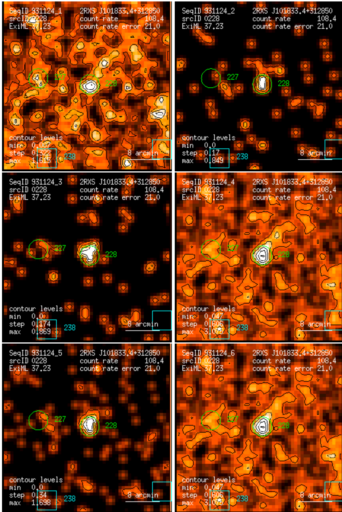
Figure 228: RASS 931124: detection 0228: band rate images, Gaussian filter: (1) PSPC channels 11 – 41, (2) 52 – 90, (3) 91 – 201, (4) 11 – 235, (5) 52 – 201, (6) 11 – 201. Broad band rates in counts/ks. Band rate contour levels in counts/ks/arcmin 2 .
