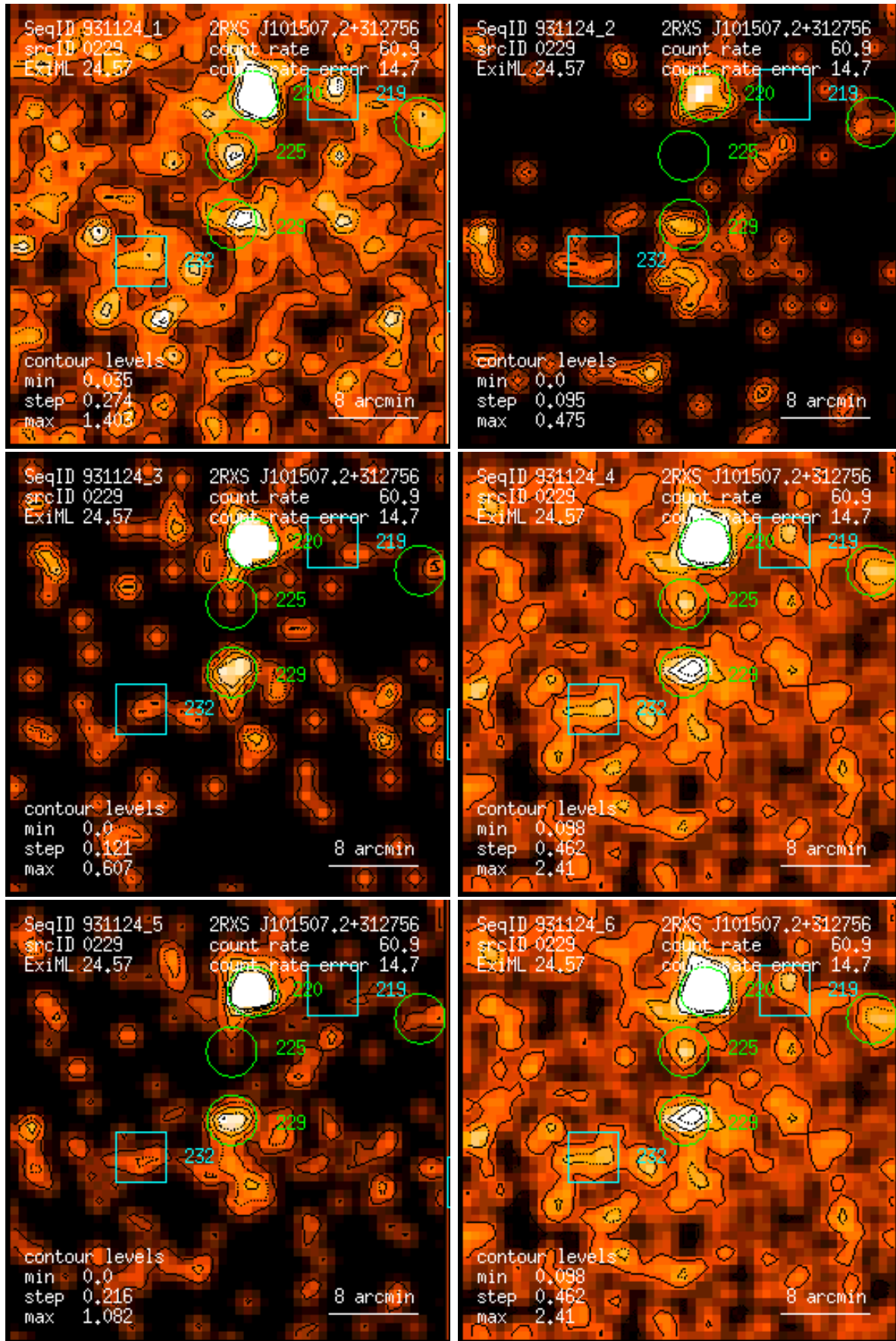
Figure 229: RASS 931124: detection 0229: band rate images, Gaussian filter: (1) PSPC channels 11 – 41, (2) 52 – 90, (3) 91 – 201, (4) 11 – 235, (5) 52 – 201, (6) 11 – 201. Broad band rates in counts/ks. Band rate contour levels in counts/ks/arcmin 2 .
