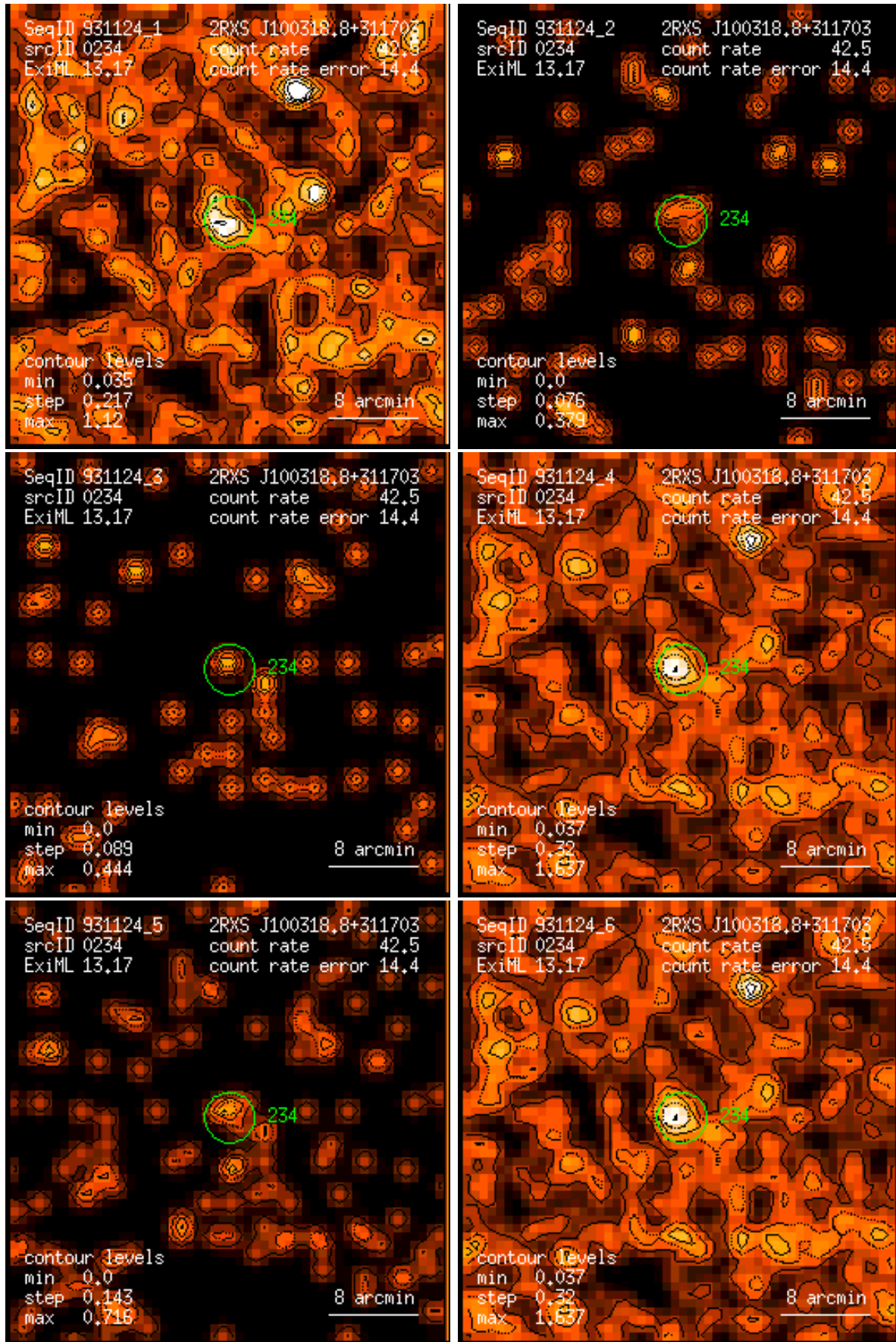
Figure 234: RASS 931124: detection 0234: band rate images, Gaussian filter: (1) PSPC channels 11 – 41, (2) 52 – 90, (3) 91 – 201, (4) 11 – 235, (5) 52 – 201, (6) 11 – 201. Broad band rates in counts/ks. Band rate contour levels in counts/ks/arcmin 2 .
