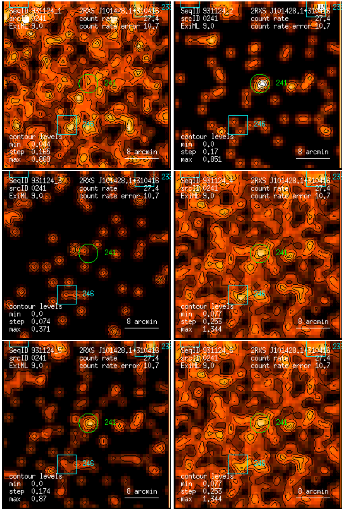
Figure 241: RASS 931124: detection 0241: band rate images, Gaussian filter: (1) PSPC channels 11 – 41, (2) 52 – 90, (3) 91 – 201, (4) 11 – 235, (5) 52 – 201, (6) 11 – 201. Broad band rates in counts/ks. Band rate contour levels in counts/ks/arcmin 2 .
