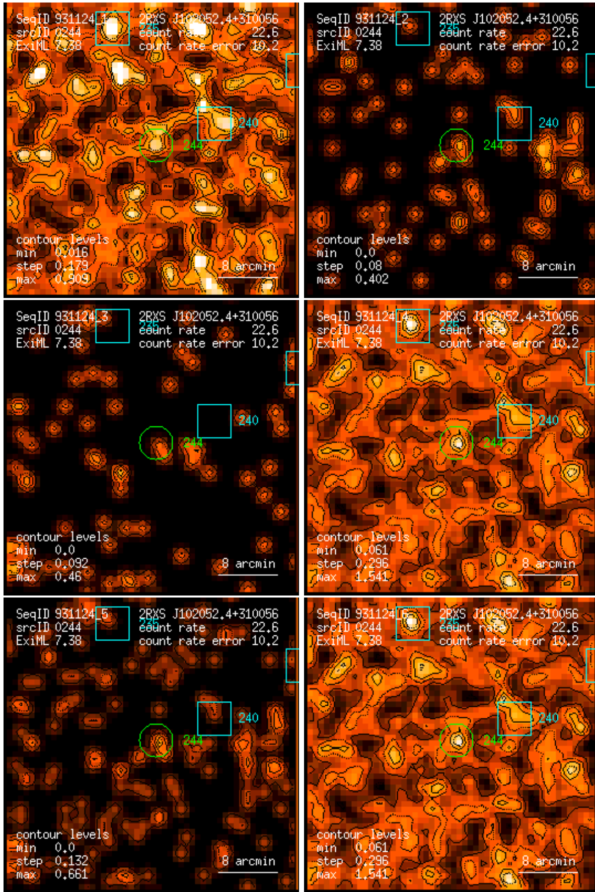
Figure 244: RASS 931124: detection 0244: band rate images, Gaussian filter: (1) PSPC channels 11 – 41, (2) 52 – 90, (3) 91 – 201, (4) 11 – 235, (5) 52 – 201, (6) 11 – 201. Broad band rates in counts/ks. Band rate contour levels in counts/ks/arcmin 2 .
