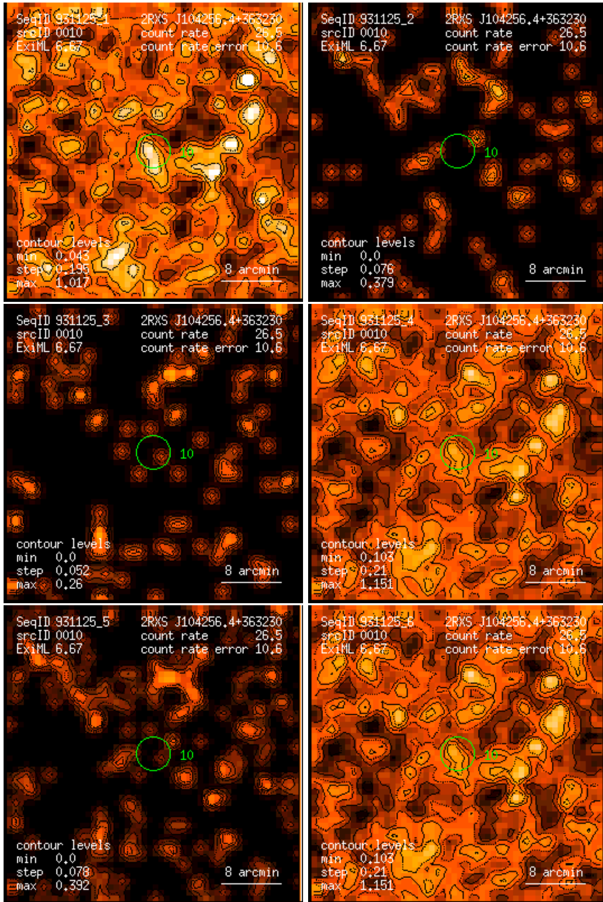
Figure 10: RASS 931125: detection 0010: band rate images, Gaussian filter: (1) PSPC channels 11 – 41, (2) 52 – 90, (3) 91 – 201, (4) 11 – 235, (5) 52 – 201, (6) 11 – 201. Broad band rates in counts/ks. Band rate contour levels in counts/ks/arcmin 2 .
