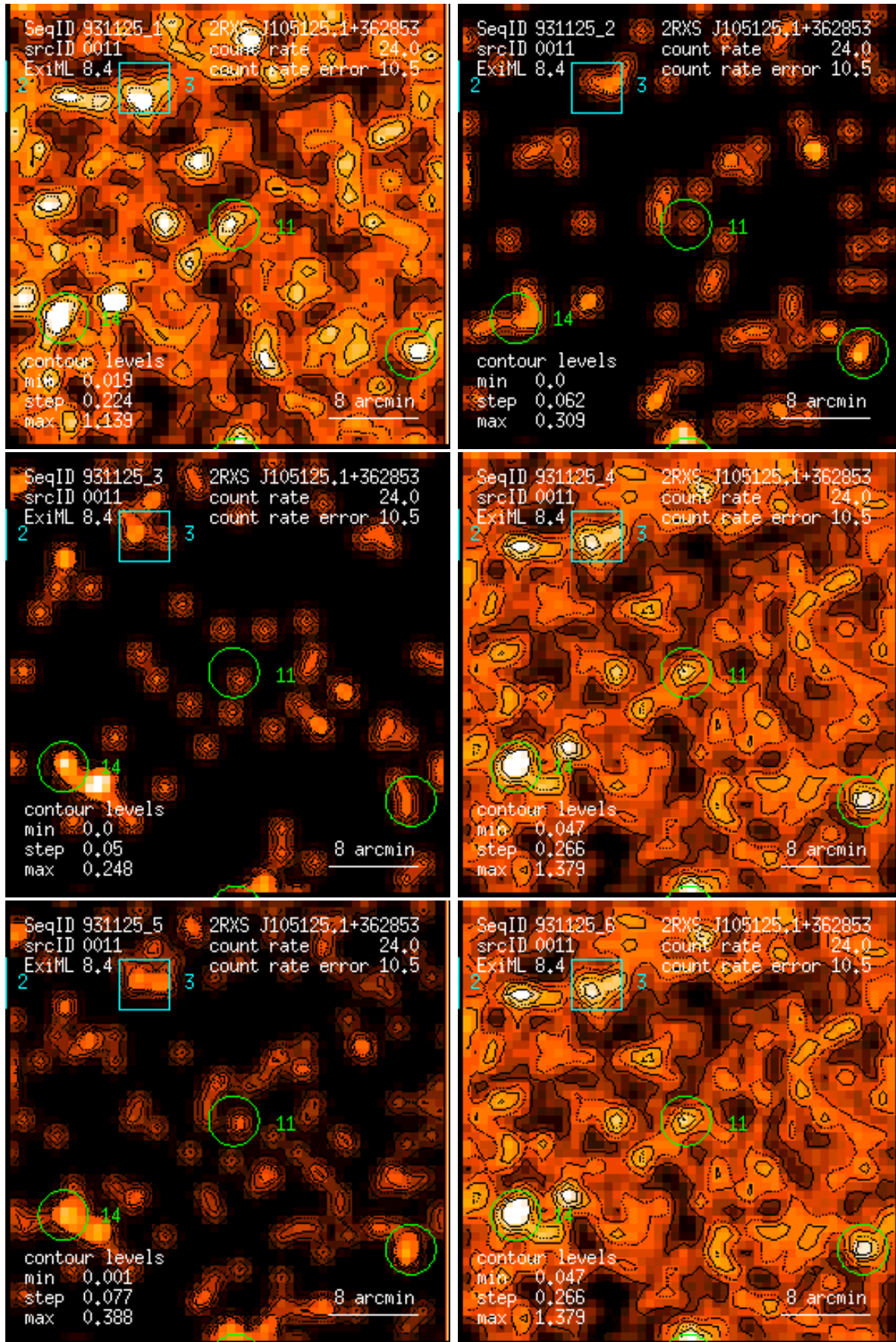
Figure 11: RASS 931125: detection 0011: band rate images, Gaussian filter: (1) PSPC channels 11 – 41, (2) 52 – 90, (3) 91 – 201, (4) 11 – 235, (5) 52 – 201, (6) 11 – 201. Broad band rates in counts/ks. Band rate contour levels in counts/ks/arcmin 2 .
