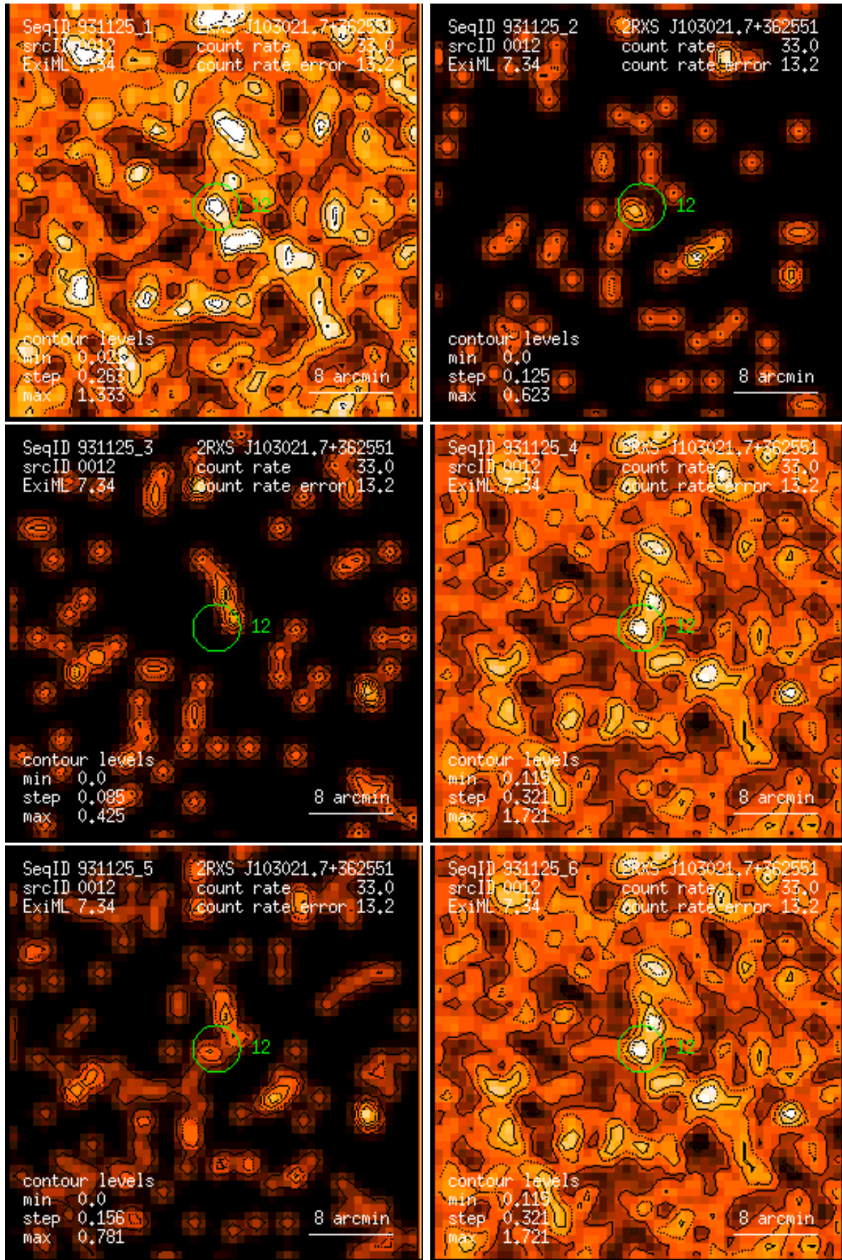
Figure 12: RASS 931125: detection 0012: band rate images, Gaussian filter: (1) PSPC channels 11 – 41, (2) 52 – 90, (3) 91 – 201, (4) 11 – 235, (5) 52 – 201, (6) 11 – 201. Broad band rates in counts/ks. Band rate contour levels in counts/ks/arcmin 2 .
