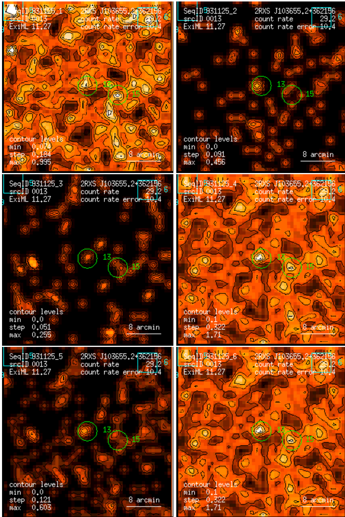
Figure 13: RASS 931125: detection 0013: band rate images, Gaussian filter: (1) PSPC channels 11 – 41, (2) 52 – 90, (3) 91 – 201, (4) 11 – 235, (5) 52 – 201, (6) 11 – 201. Broad band rates in counts/ks. Band rate contour levels in counts/ks/arcmin 2 .
