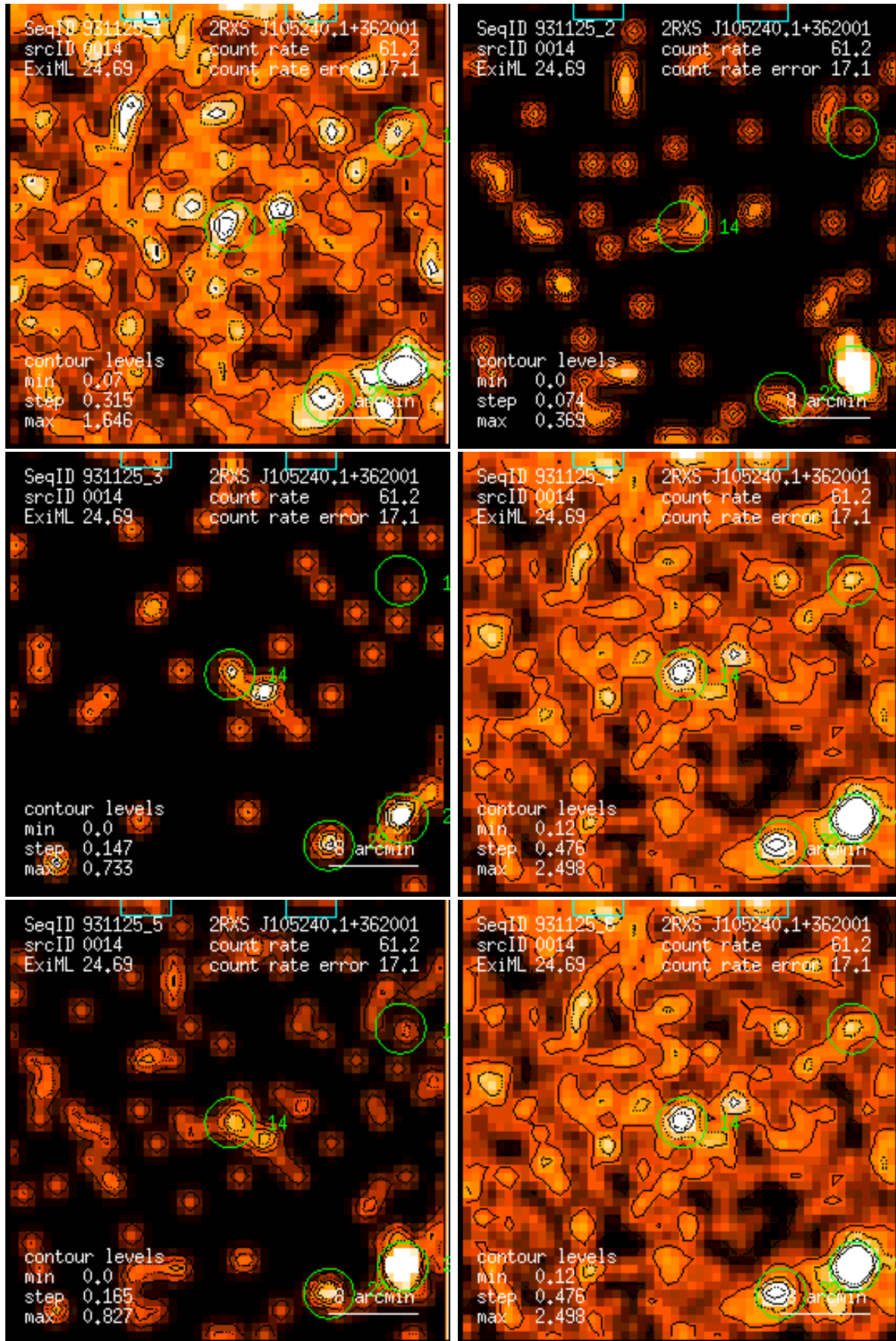
Figure 14: RASS 931125: detection 0014: band rate images, Gaussian filter: (1) PSPC channels 11 – 41, (2) 52 – 90, (3) 91 – 201, (4) 11 – 235, (5) 52 – 201, (6) 11 – 201. Broad band rates in counts/ks. Band rate contour levels in counts/ks/arcmin 2 .
