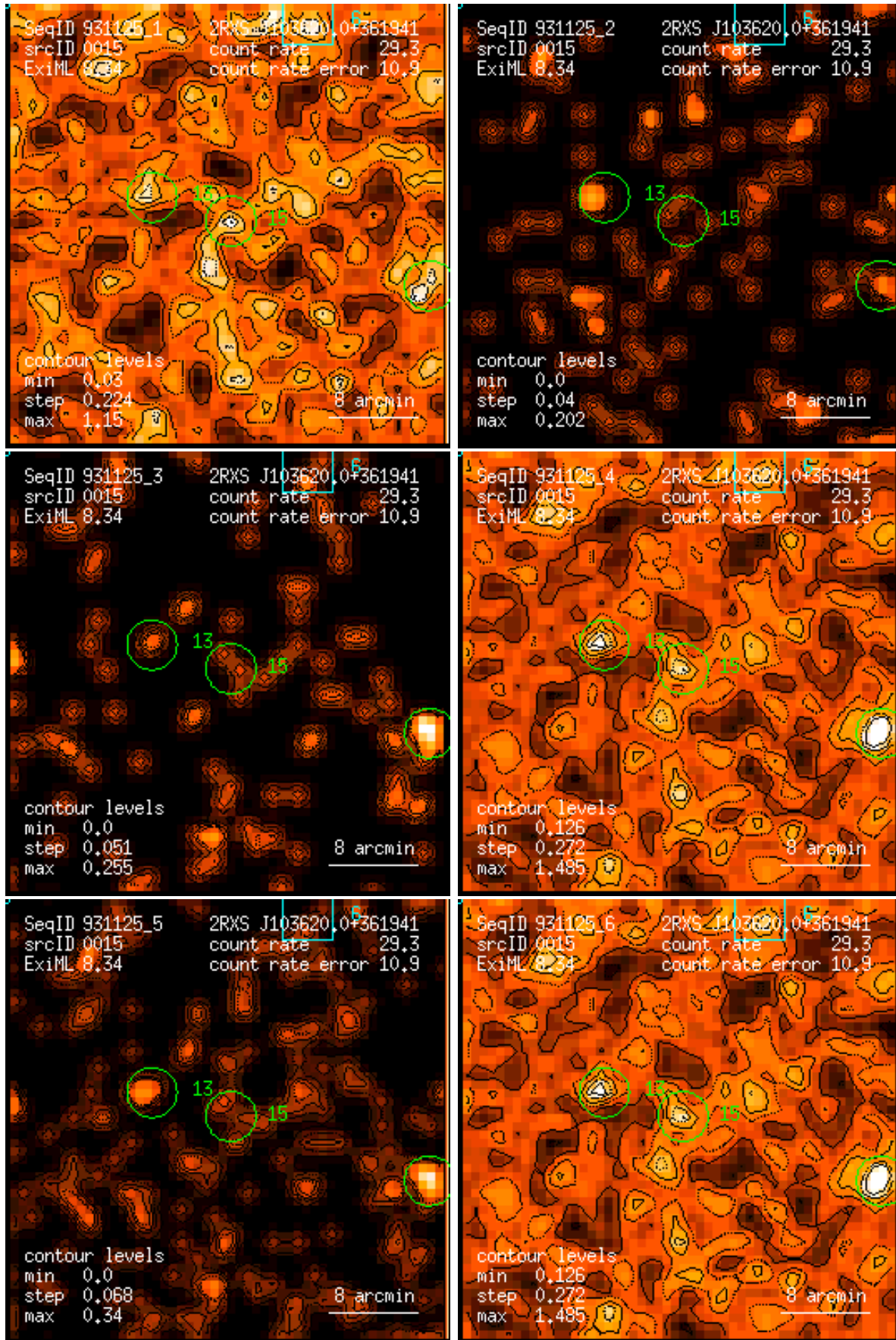
Figure 15: RASS 931125: detection 0015: band rate images, Gaussian filter: (1) PSPC channels 11 – 41, (2) 52 – 90, (3) 91 – 201, (4) 11 – 235, (5) 52 – 201, (6) 11 – 201. Broad band rates in counts/ks. Band rate contour levels in counts/ks/arcmin 2 .
