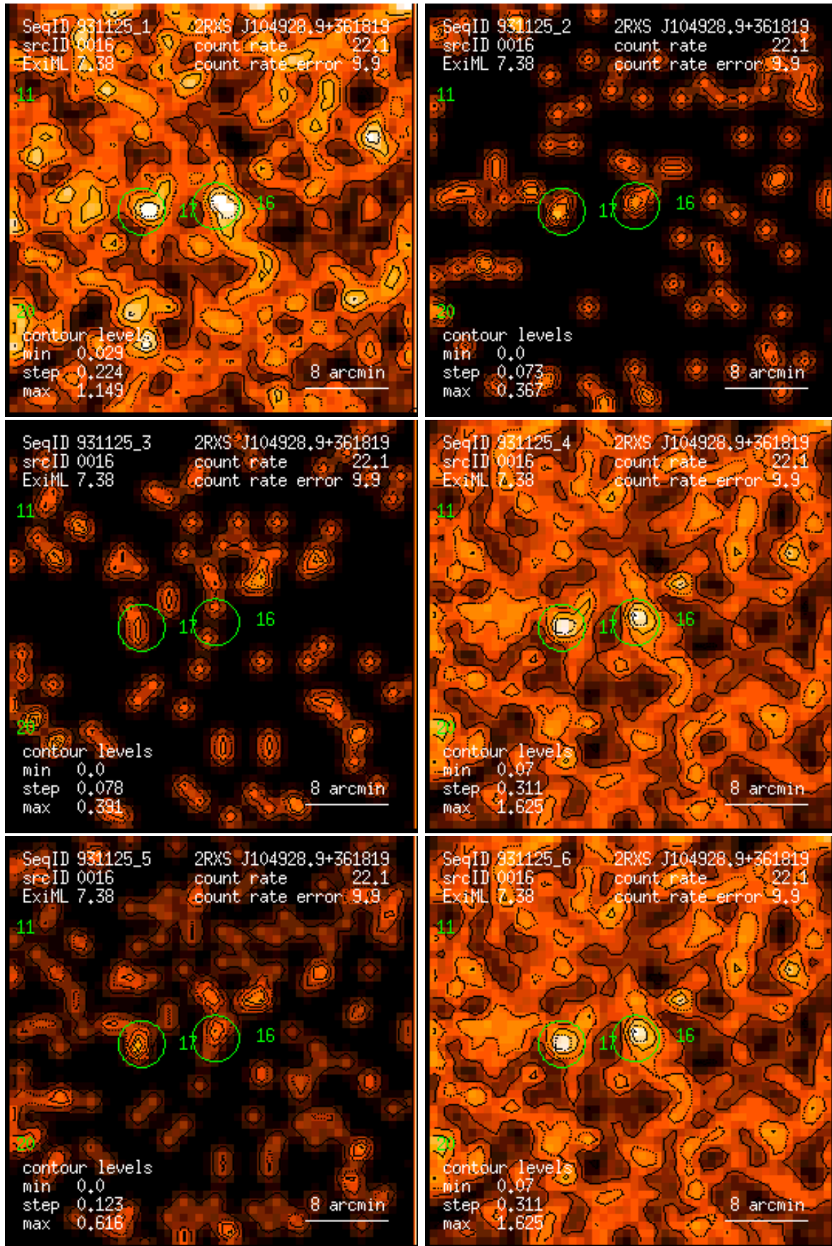
Figure 16: RASS 931125: detection 0016: band rate images, Gaussian filter: (1) PSPC channels 11 – 41, (2) 52 – 90, (3) 91 – 201, (4) 11 – 235, (5) 52 – 201, (6) 11 – 201. Broad band rates in counts/ks. Band rate contour levels in counts/ks/arcmin 2 .
