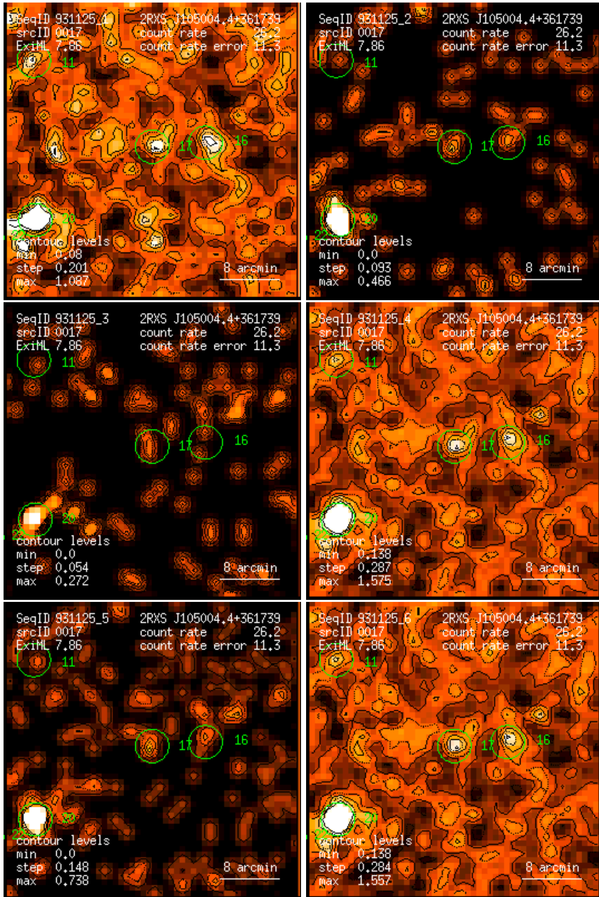
Figure 17: RASS 931125: detection 0017: band rate images, Gaussian filter: (1) PSPC channels 11 – 41, (2) 52 – 90, (3) 91 – 201, (4) 11 – 235, (5) 52 – 201, (6) 11 – 201. Broad band rates in counts/ks. Band rate contour levels in counts/ks/arcmin 2 .
