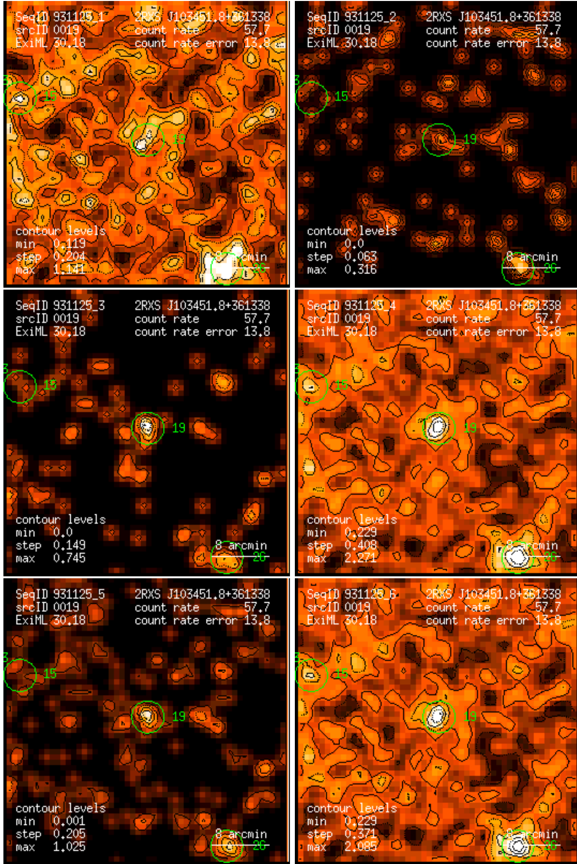
Figure 19: RASS 931125: detection 0019: band rate images, Gaussian filter: (1) PSPC channels 11 – 41, (2) 52 – 90, (3) 91 – 201, (4) 11 – 235, (5) 52 – 201, (6) 11 – 201. Broad band rates in counts/ks. Band rate contour levels in counts/ks/arcmin 2 .
