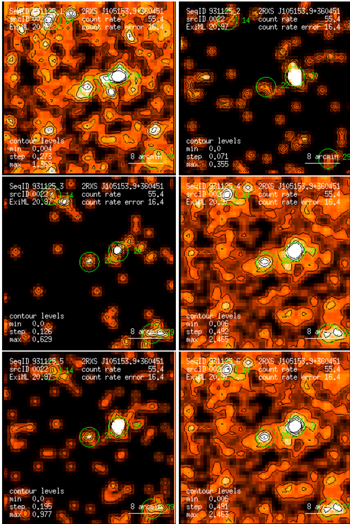
Figure 22: RASS 931125: detection 0022: band rate images, Gaussian filter: (1) PSPC channels 11 – 41, (2) 52 – 90, (3) 91 – 201, (4) 11 – 235, (5) 52 – 201, (6) 11 – 201. Broad band rates in counts/ks. Band rate contour levels in counts/ks/arcmin 2 .
