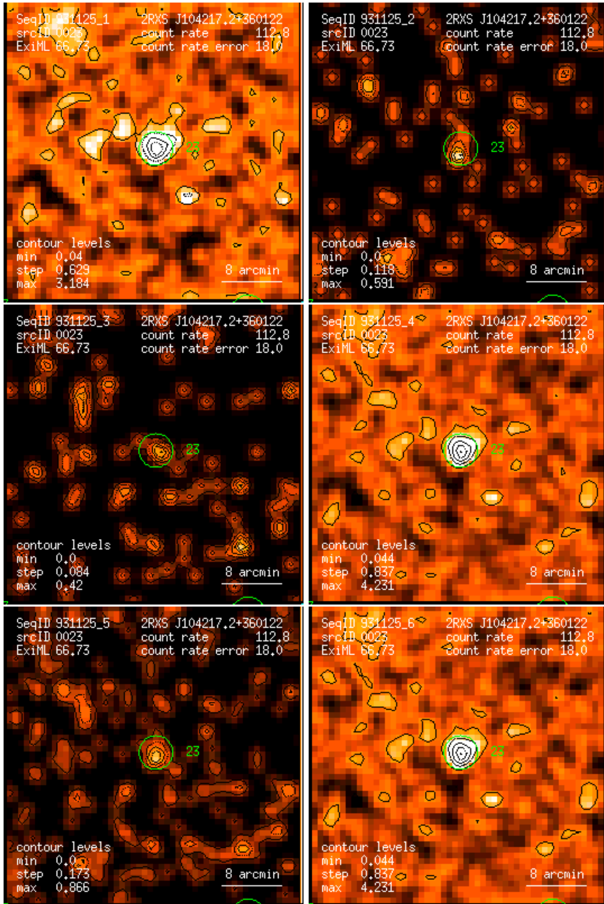
Figure 23: RASS 931125: detection 0023: band rate images, Gaussian filter: (1) PSPC channels 11 – 41, (2) 52 – 90, (3) 91 – 201, (4) 11 – 235, (5) 52 – 201, (6) 11 – 201. Broad band rates in counts/ks. Band rate contour levels in counts/ks/arcmin 2 .
