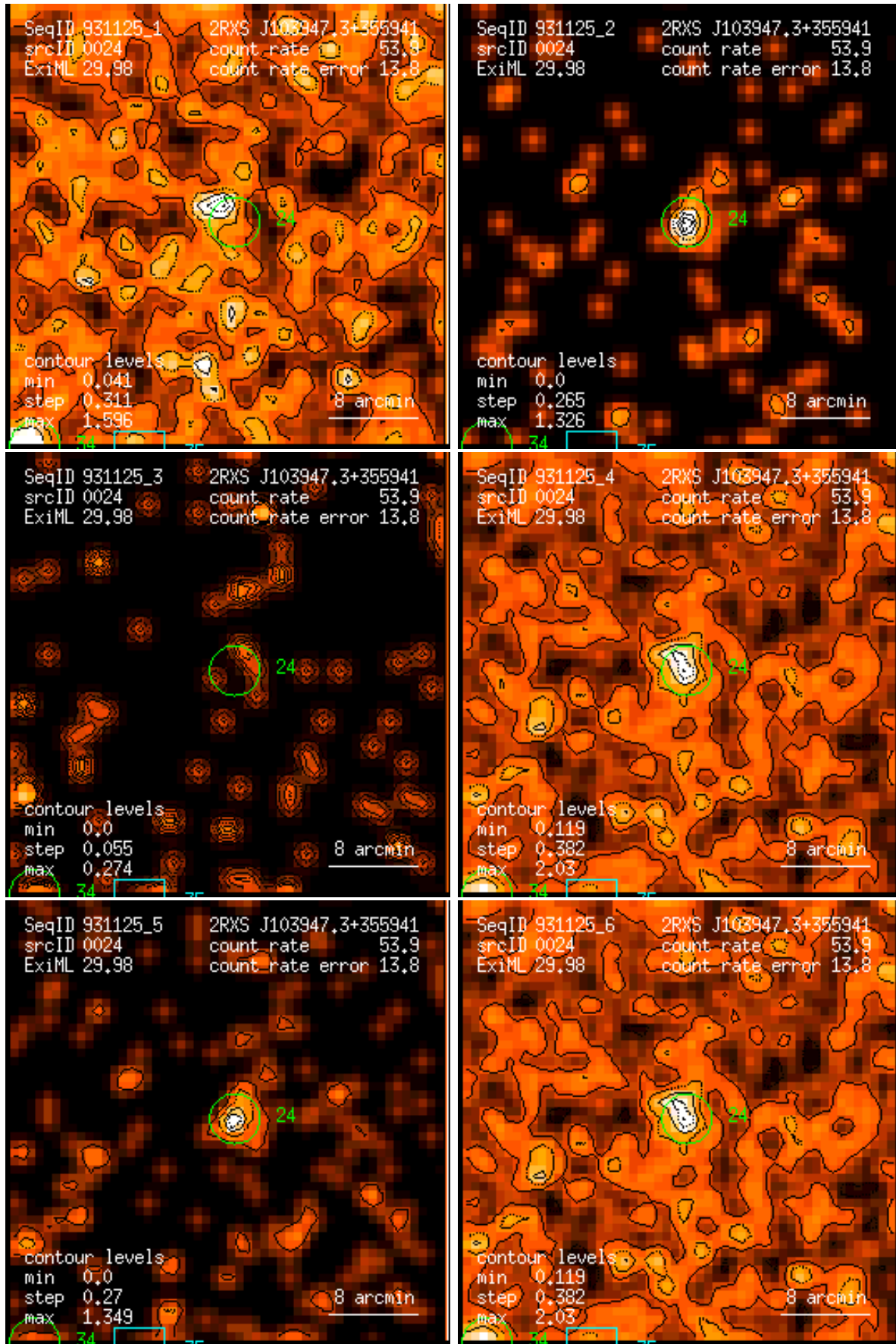
Figure 24: RASS 931125: detection 0024: band rate images, Gaussian filter: (1) PSPC channels 11 – 41, (2) 52 – 90, (3) 91 – 201, (4) 11 – 235, (5) 52 – 201, (6) 11 – 201. Broad band rates in counts/ks. Band rate contour levels in counts/ks/arcmin 2 .
