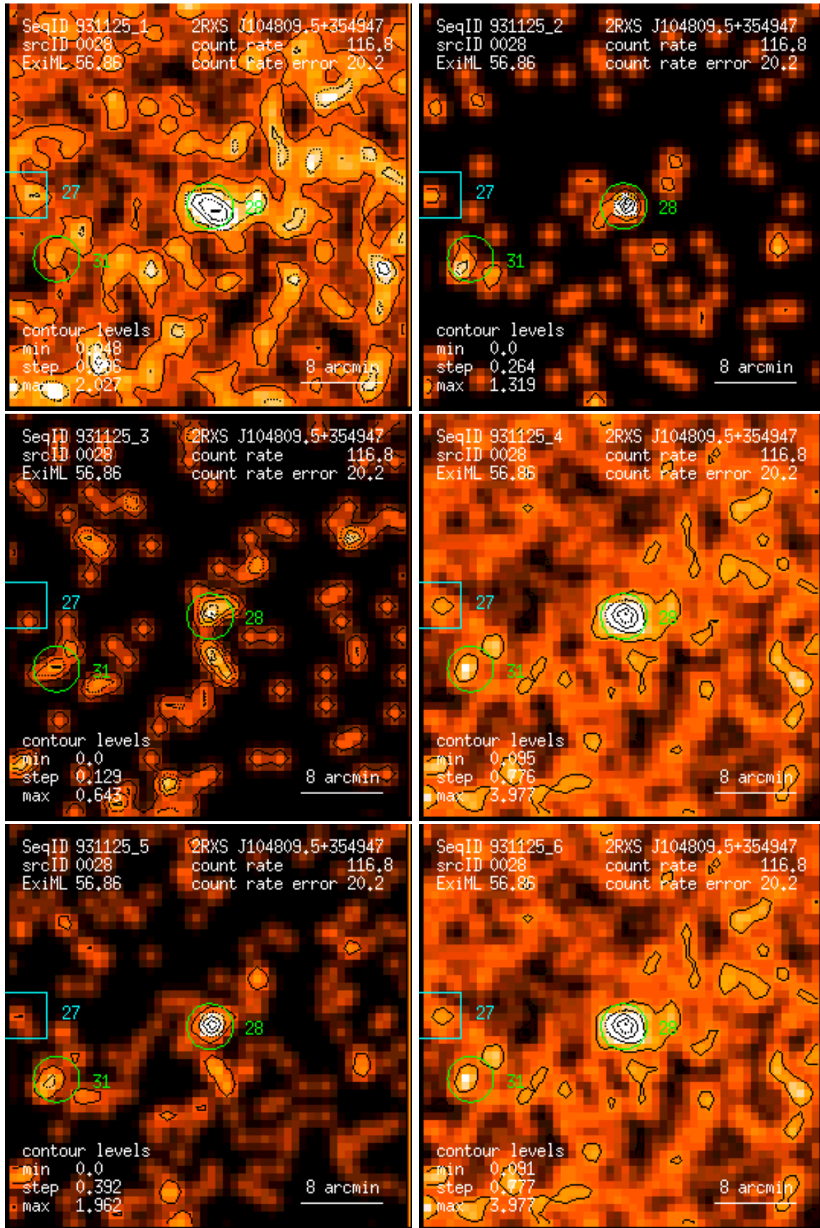
Figure 28: RASS 931125: detection 0028: band rate images, Gaussian filter: (1) PSPC channels 11 – 41, (2) 52 – 90, (3) 91 – 201, (4) 11 – 235, (5) 52 – 201, (6) 11 – 201. Broad band rates in counts/ks. Band rate contour levels in counts/ks/arcmin 2 .
