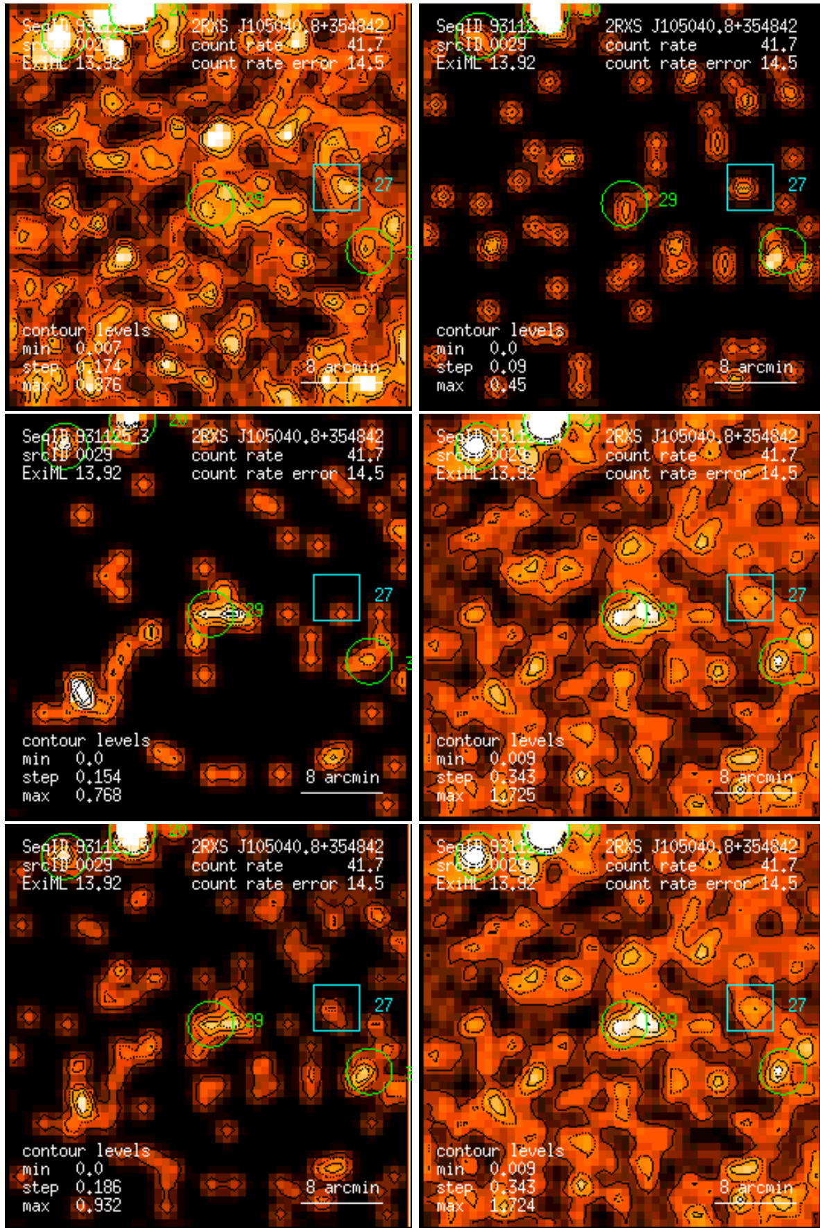
Figure 29: RASS 931125: detection 0029: band rate images, Gaussian filter: (1) PSPC channels 11 – 41, (2) 52 – 90, (3) 91 – 201, (4) 11 – 235, (5) 52 – 201, (6) 11 – 201. Broad band rates in counts/ks. Band rate contour levels in counts/ks/arcmin 2 .
