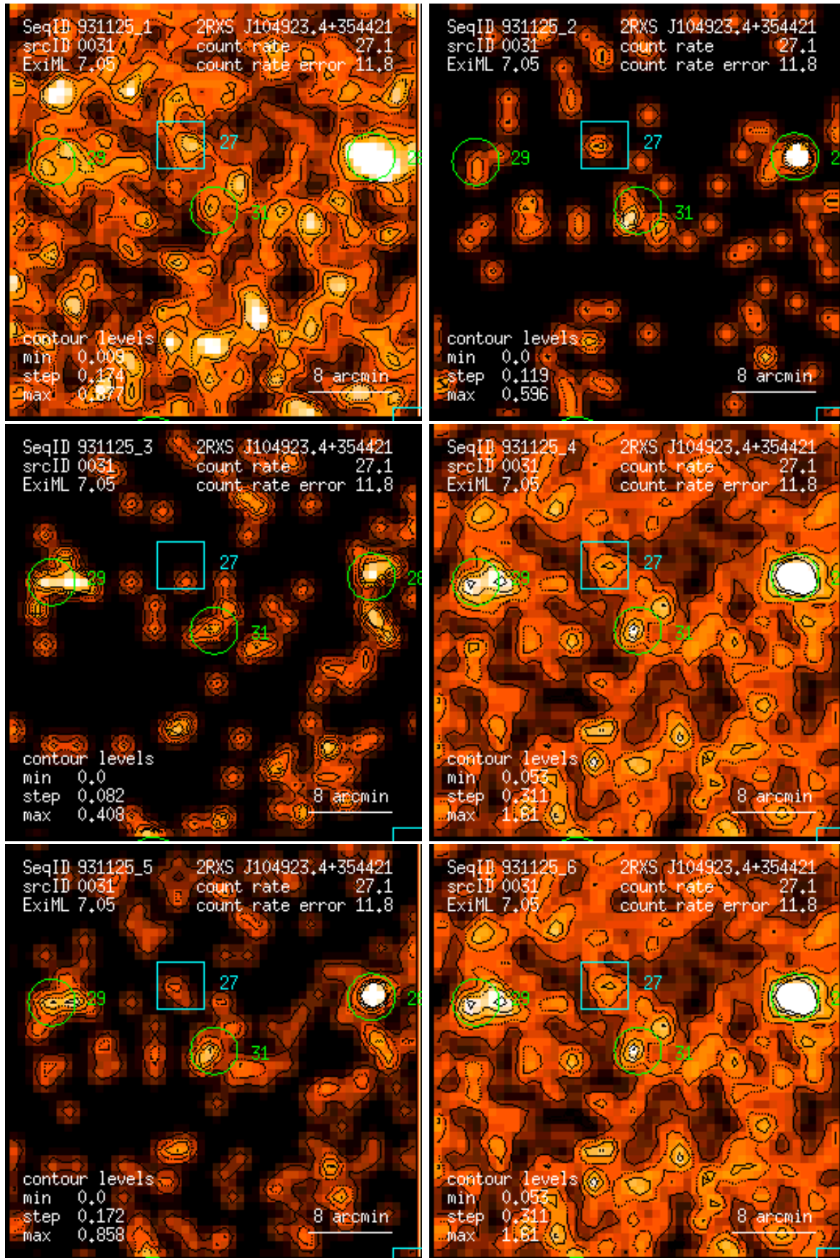
Figure 31: RASS 931125: detection 0031: band rate images, Gaussian filter: (1) PSPC channels 11 – 41, (2) 52 – 90, (3) 91 – 201, (4) 11 – 235, (5) 52 – 201, (6) 11 – 201. Broad band rates in counts/ks. Band rate contour levels in counts/ks/arcmin 2 .
