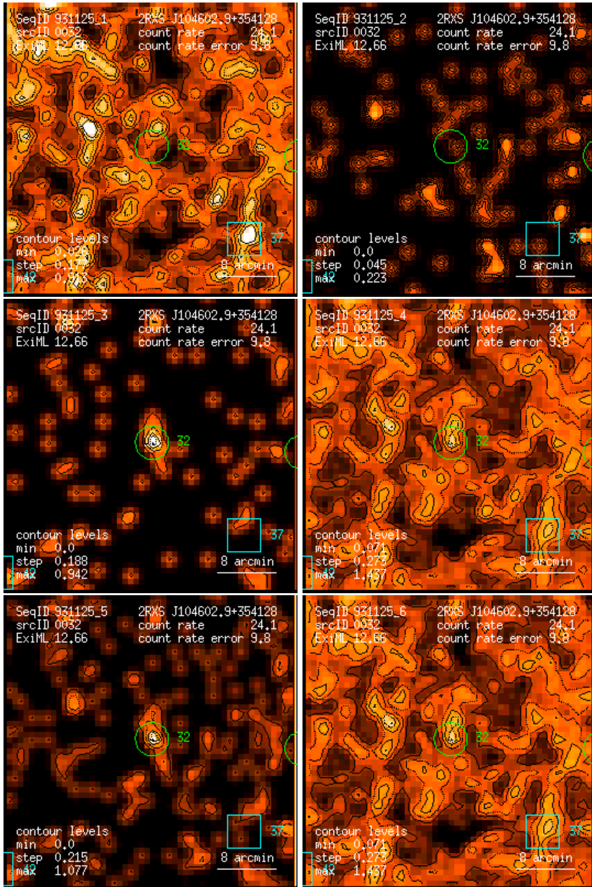
Figure 32: RASS 931125: detection 0032: band rate images, Gaussian filter: (1) PSPC channels 11 – 41, (2) 52 – 90, (3) 91 – 201, (4) 11 – 235, (5) 52 – 201, (6) 11 – 201. Broad band rates in counts/ks. Band rate contour levels in counts/ks/arcmin 2 .
