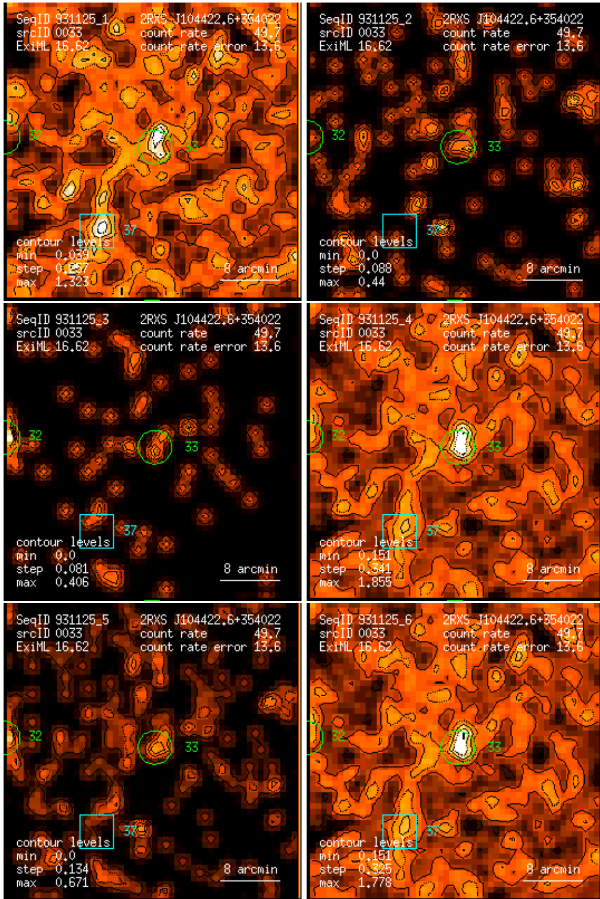
Figure 33: RASS 931125: detection 0033: band rate images, Gaussian filter: (1) PSPC channels 11 – 41, (2) 52 – 90, (3) 91 – 201, (4) 11 – 235, (5) 52 – 201, (6) 11 – 201. Broad band rates in counts/ks. Band rate contour levels in counts/ks/arcmin 2 .
