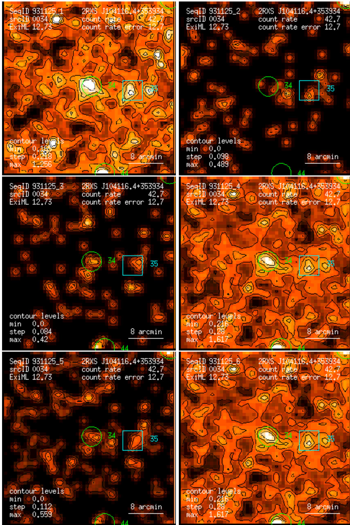
Figure 34: RASS 931125: detection 0034: band rate images, Gaussian filter: (1) PSPC channels 11 – 41, (2) 52 – 90, (3) 91 – 201, (4) 11 – 235, (5) 52 – 201, (6) 11 – 201. Broad band rates in counts/ks. Band rate contour levels in counts/ks/arcmin 2 .
