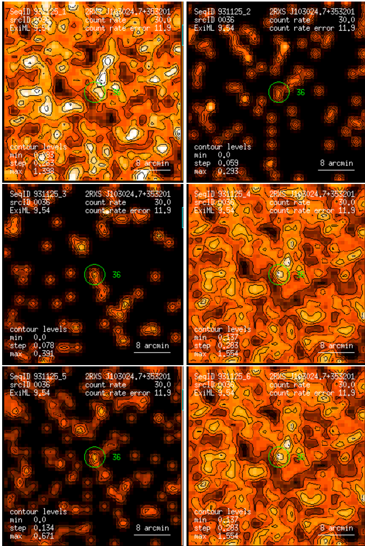
Figure 36: RASS 931125: detection 0036: band rate images, Gaussian filter: (1) PSPC channels 11 – 41, (2) 52 – 90, (3) 91 – 201, (4) 11 – 235, (5) 52 – 201, (6) 11 – 201. Broad band rates in counts/ks. Band rate contour levels in counts/ks/arcmin 2 .
