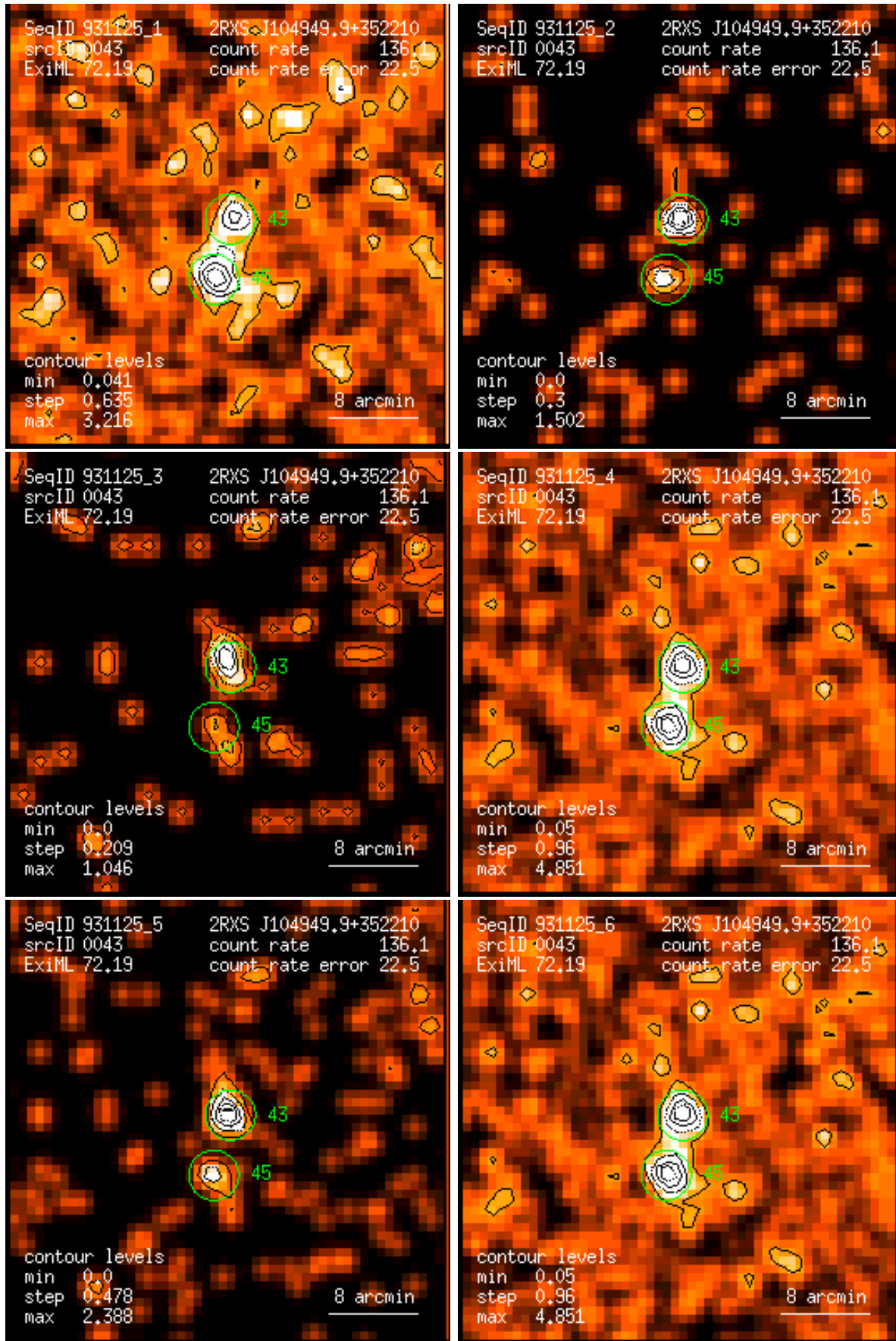
Figure 43: RASS 931125: detection 0043: band rate images, Gaussian filter: (1) PSPC channels 11 – 41, (2) 52 – 90, (3) 91 – 201, (4) 11 – 235, (5) 52 – 201, (6) 11 – 201. Broad band rates in counts/ks. Band rate contour levels in counts/ks/arcmin 2 .
