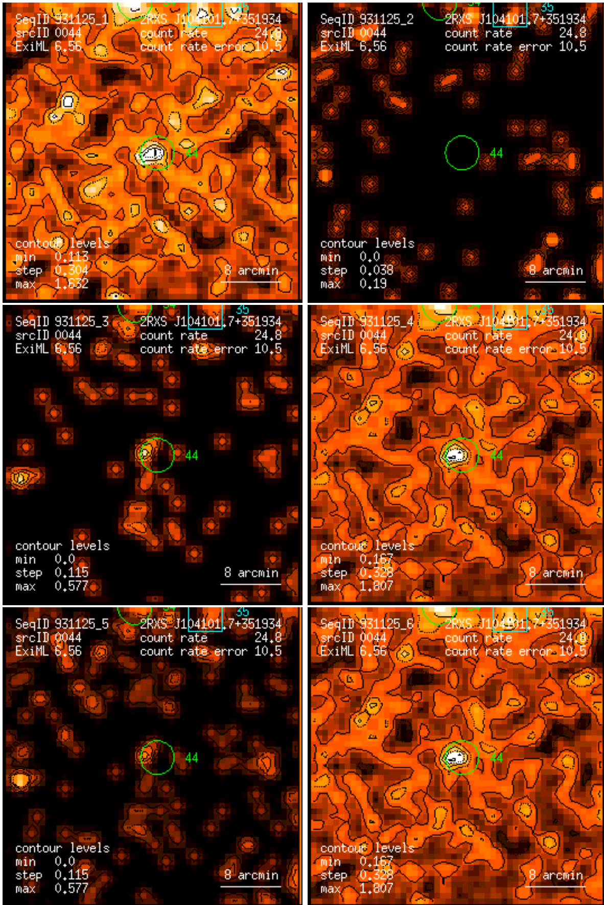
Figure 44: RASS 931125: detection 0044: band rate images, Gaussian filter: (1) PSPC channels 11 – 41, (2) 52 – 90, (3) 91 – 201, (4) 11 – 235, (5) 52 – 201, (6) 11 – 201. Broad band rates in counts/ks. Band rate contour levels in counts/ks/arcmin 2 .
