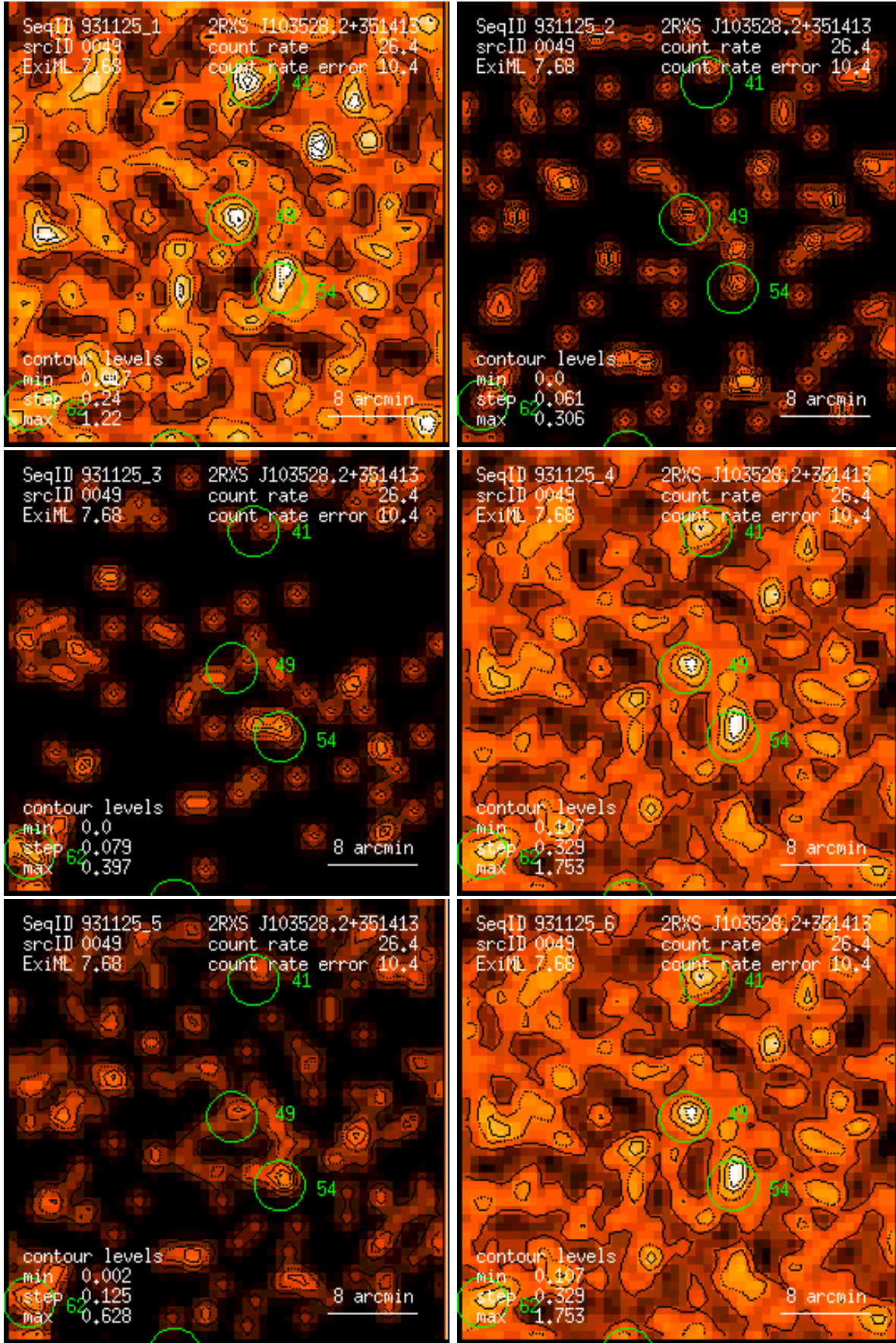
Figure 49: RASS 931125: detection 0049: band rate images, Gaussian filter: (1) PSPC channels 11 – 41, (2) 52 – 90, (3) 91 – 201, (4) 11 – 235, (5) 52 – 201, (6) 11 – 201. Broad band rates in counts/ks. Band rate contour levels in counts/ks/arcmin 2 .
