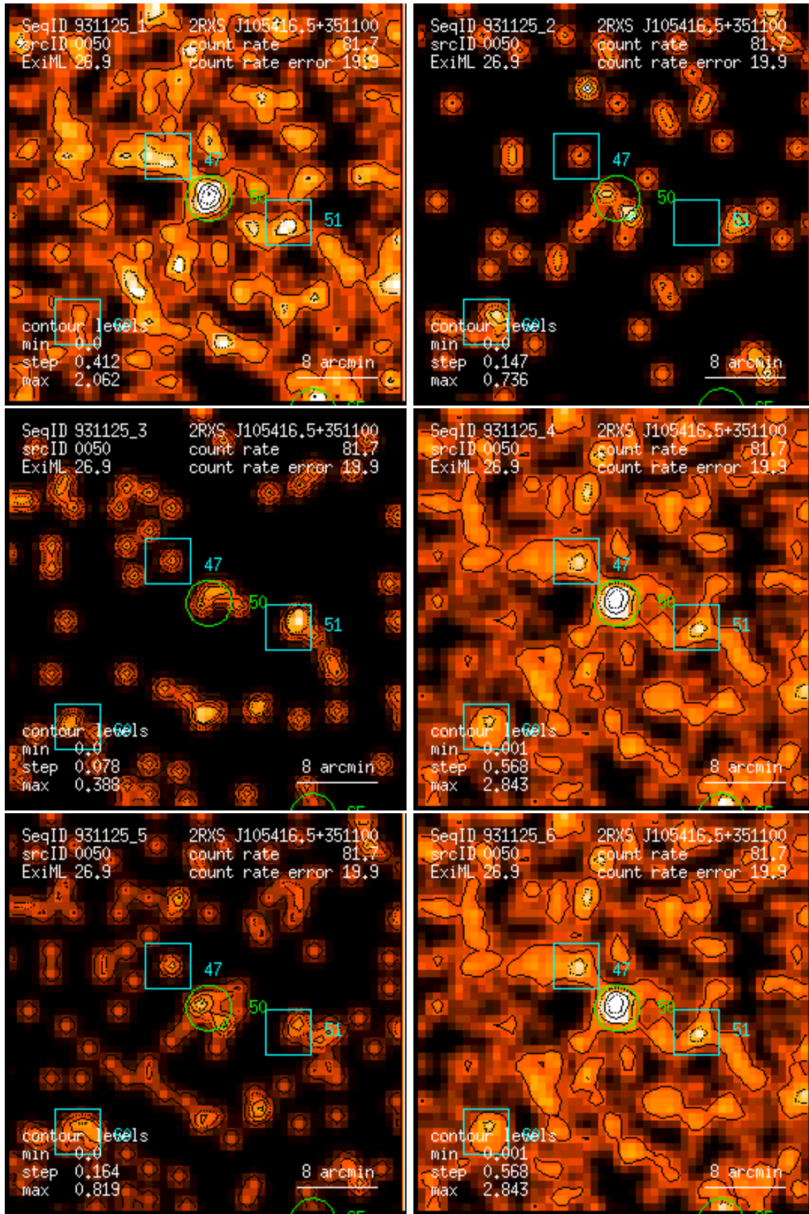
Figure 50: RASS 931125: detection 0050: band rate images, Gaussian filter: (1) PSPC channels 11 – 41, (2) 52 – 90, (3) 91 – 201, (4) 11 – 235, (5) 52 – 201, (6) 11 – 201. Broad band rates in counts/ks. Band rate contour levels in counts/ks/arcmin 2 .
