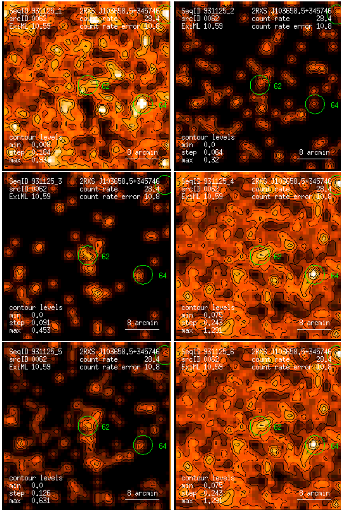
Figure 62: RASS 931125: detection 0062: band rate images, Gaussian filter: (1) PSPC channels 11 – 41, (2) 52 – 90, (3) 91 – 201, (4) 11 – 235, (5) 52 – 201, (6) 11 – 201. Broad band rates in counts/ks. Band rate contour levels in counts/ks/arcmin 2 .
