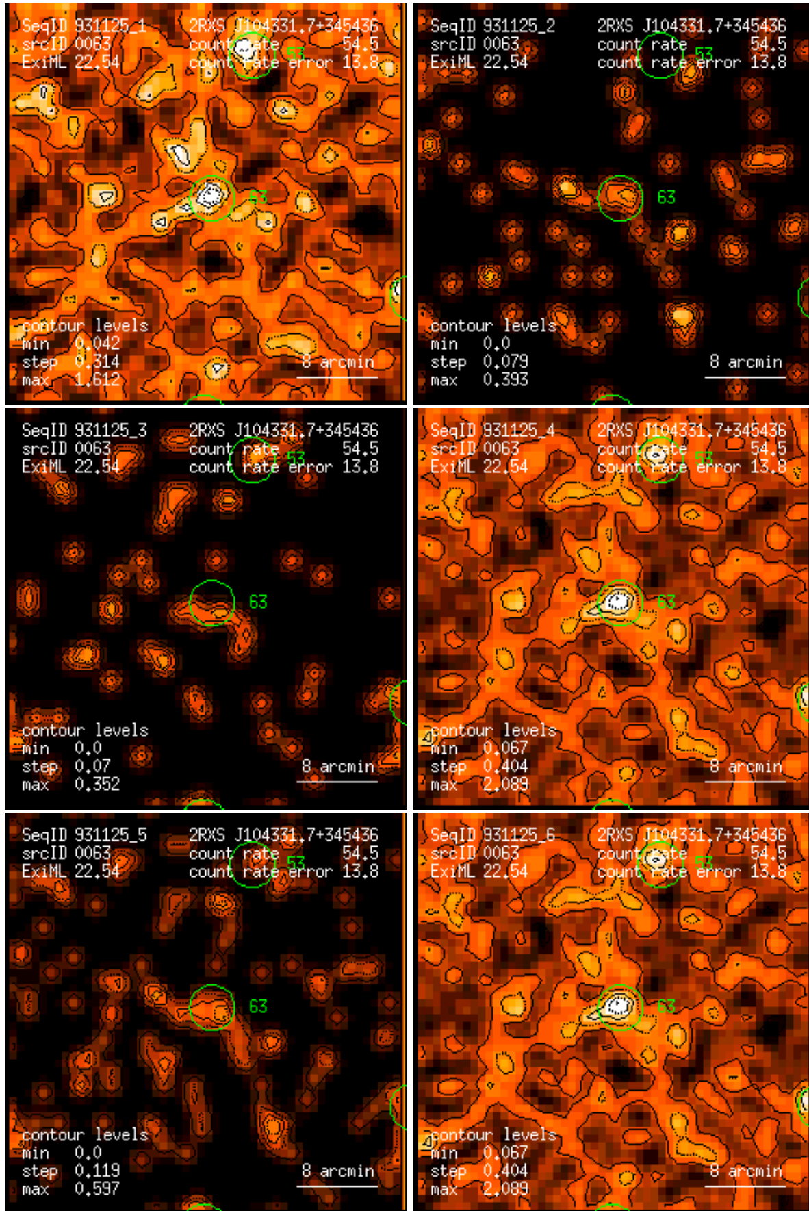
Figure 63: RASS 931125: detection 0063: band rate images, Gaussian filter: (1) PSPC channels 11 – 41, (2) 52 – 90, (3) 91 – 201, (4) 11 – 235, (5) 52 – 201, (6) 11 – 201. Broad band rates in counts/ks. Band rate contour levels in counts/ks/arcmin 2 .
