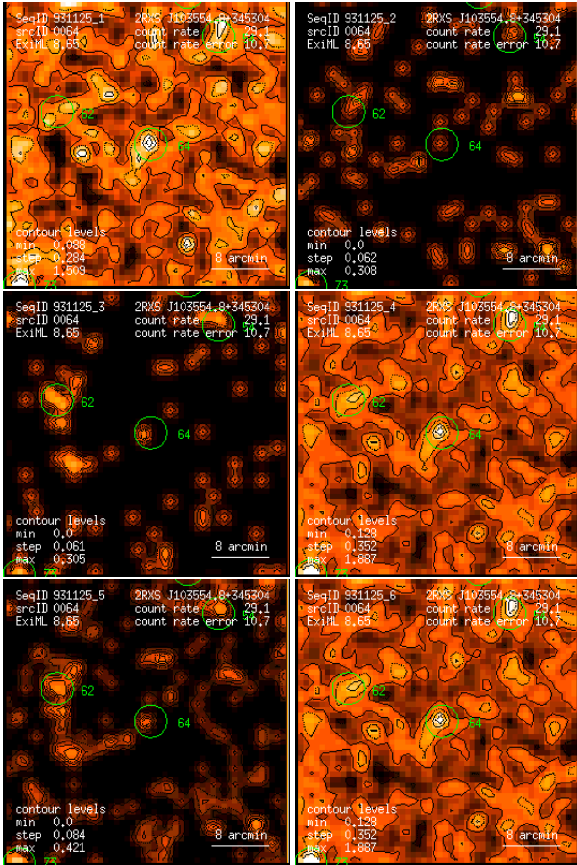
Figure 64: RASS 931125: detection 0064: band rate images, Gaussian filter: (1) PSPC channels 11 – 41, (2) 52 – 90, (3) 91 – 201, (4) 11 – 235, (5) 52 – 201, (6) 11 – 201. Broad band rates in counts/ks. Band rate contour levels in counts/ks/arcmin 2 .
