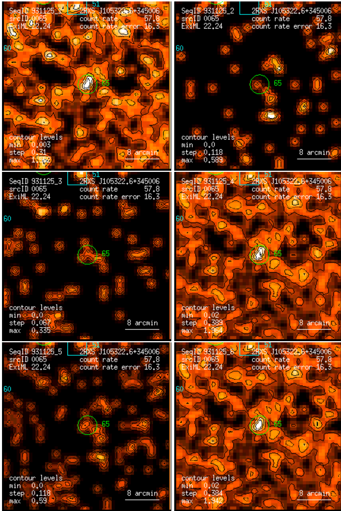
Figure 65: RASS 931125: detection 0065: band rate images, Gaussian filter: (1) PSPC channels 11 – 41, (2) 52 – 90, (3) 91 – 201, (4) 11 – 235, (5) 52 – 201, (6) 11 – 201. Broad band rates in counts/ks. Band rate contour levels in counts/ks/arcmin 2 .
