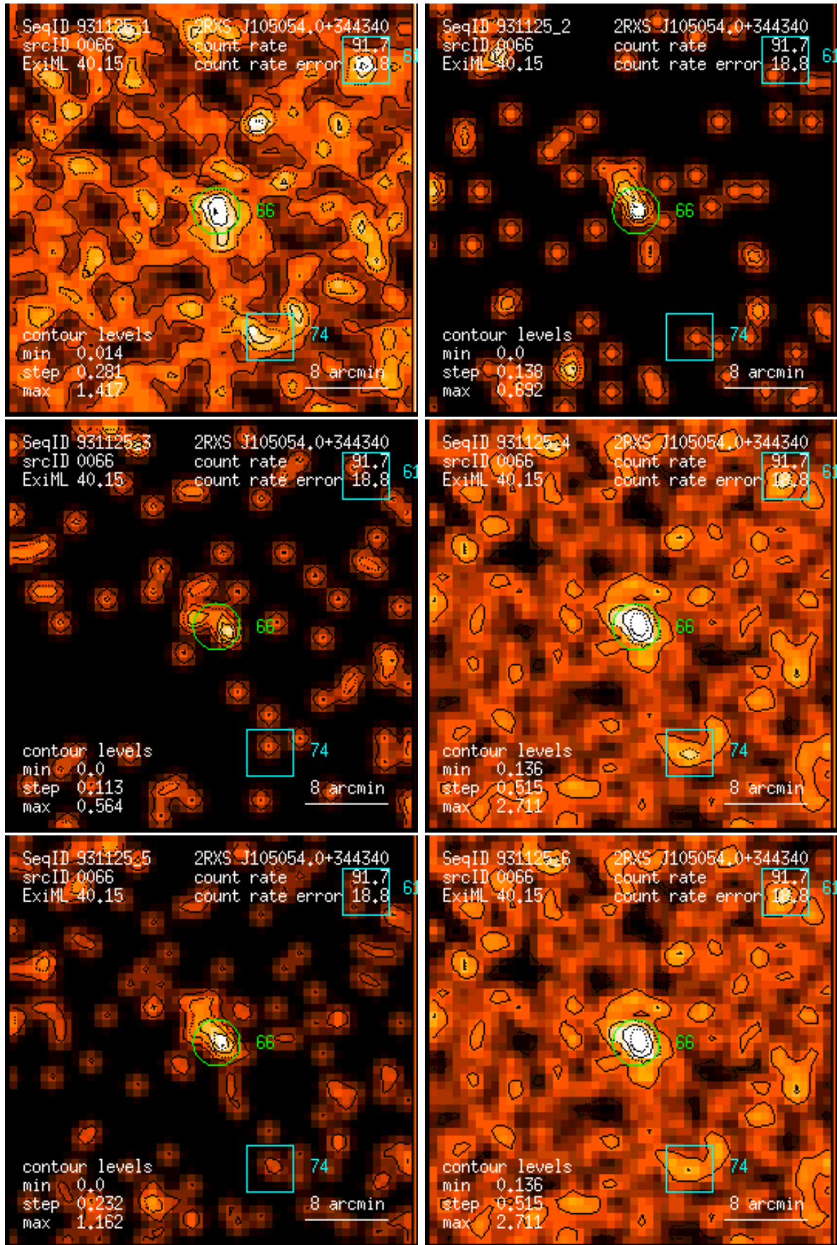
Figure 66: RASS 931125: detection 0066: band rate images, Gaussian filter: (1) PSPC channels 11 – 41, (2) 52 – 90, (3) 91 – 201, (4) 11 – 235, (5) 52 – 201, (6) 11 – 201. Broad band rates in counts/ks. Band rate contour levels in counts/ks/arcmin 2 .
