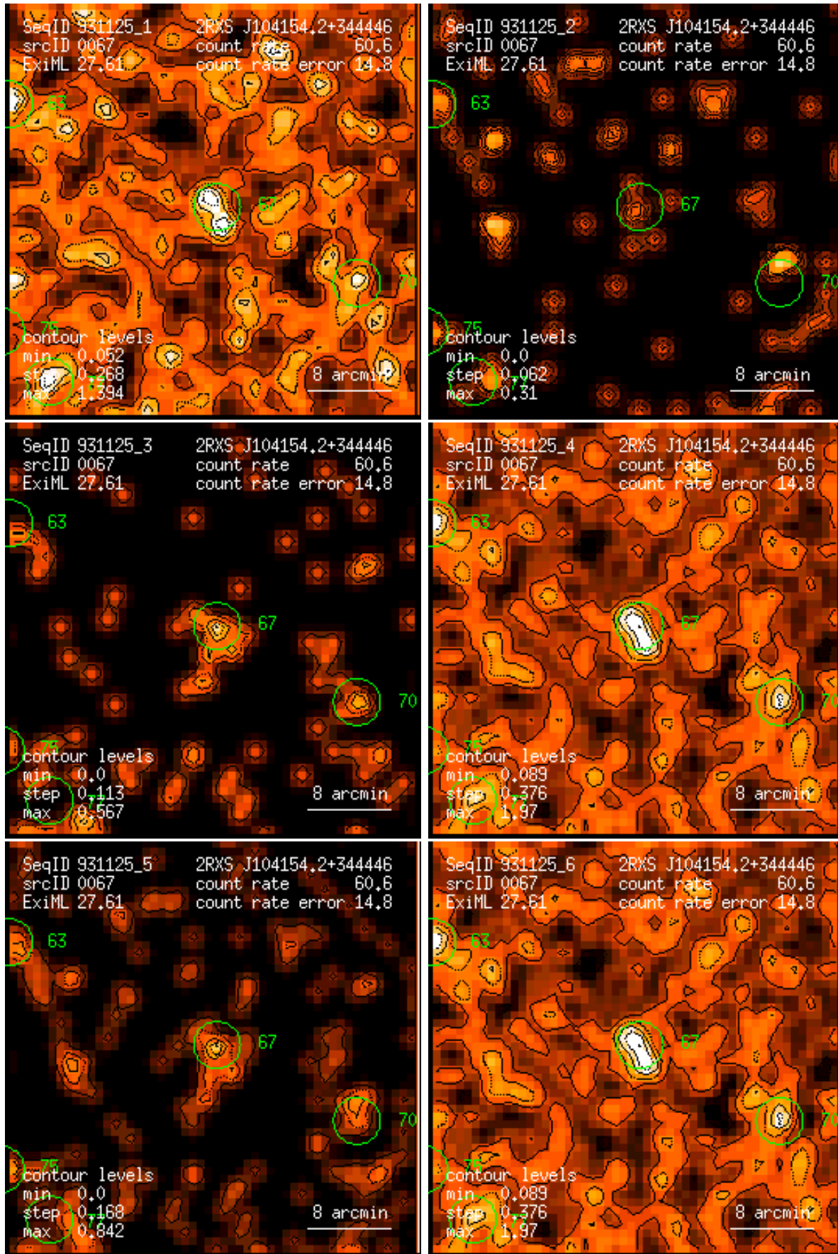
Figure 67: RASS 931125: detection 0067: band rate images, Gaussian filter: (1) PSPC channels 11 – 41, (2) 52 – 90, (3) 91 – 201, (4) 11 – 235, (5) 52 – 201, (6) 11 – 201. Broad band rates in counts/ks. Band rate contour levels in counts/ks/arcmin 2 .
