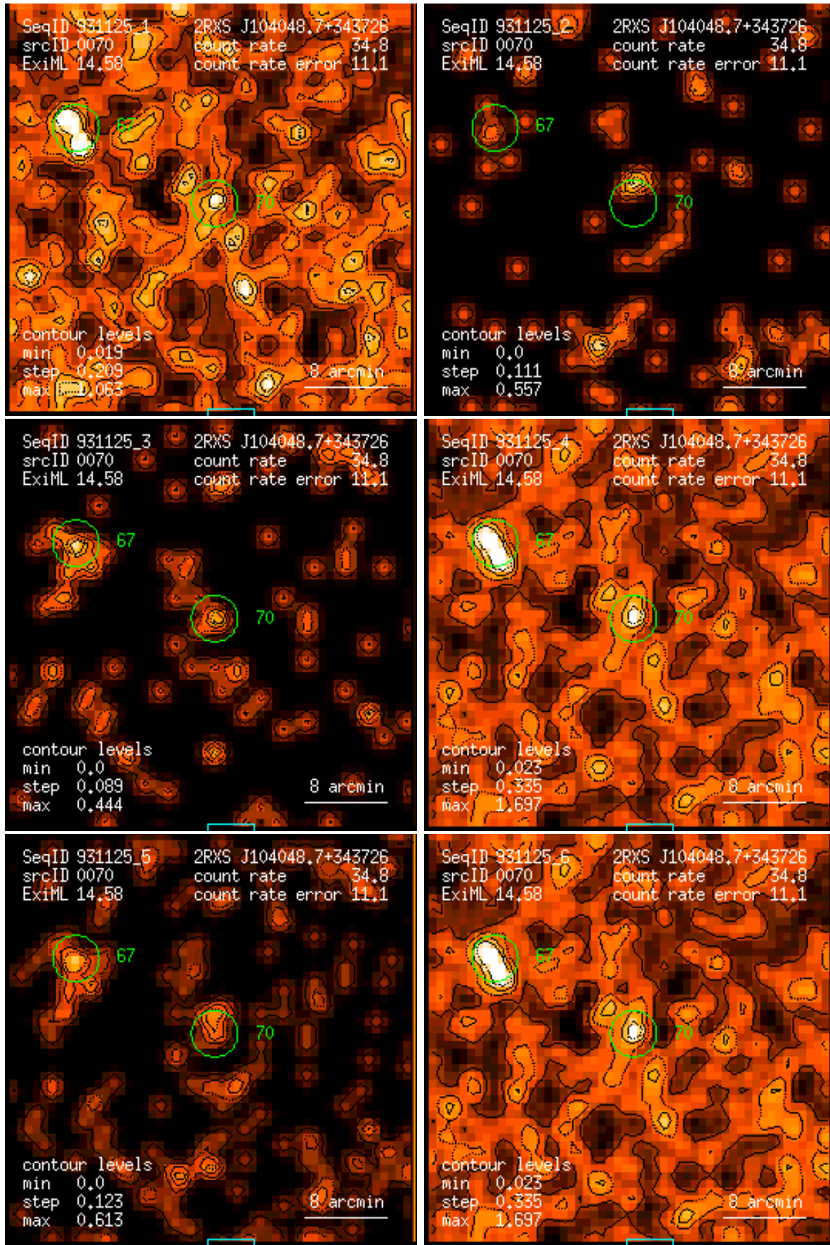
Figure 70: RASS 931125: detection 0070: band rate images, Gaussian filter: (1) PSPC channels 11 – 41, (2) 52 – 90, (3) 91 – 201, (4) 11 – 235, (5) 52 – 201, (6) 11 – 201. Broad band rates in counts/ks. Band rate contour levels in counts/ks/arcmin 2 .
