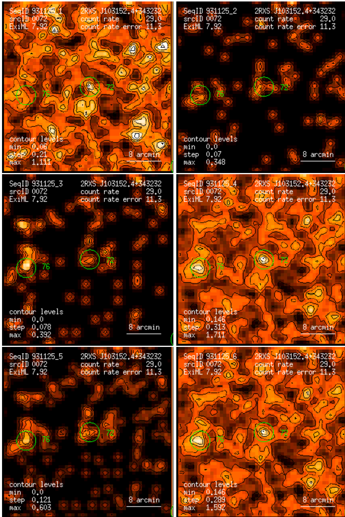
Figure 72: RASS 931125: detection 0072: band rate images, Gaussian filter: (1) PSPC channels 11 – 41, (2) 52 – 90, (3) 91 – 201, (4) 11 – 235, (5) 52 – 201, (6) 11 – 201. Broad band rates in counts/ks. Band rate contour levels in counts/ks/arcmin 2 .
