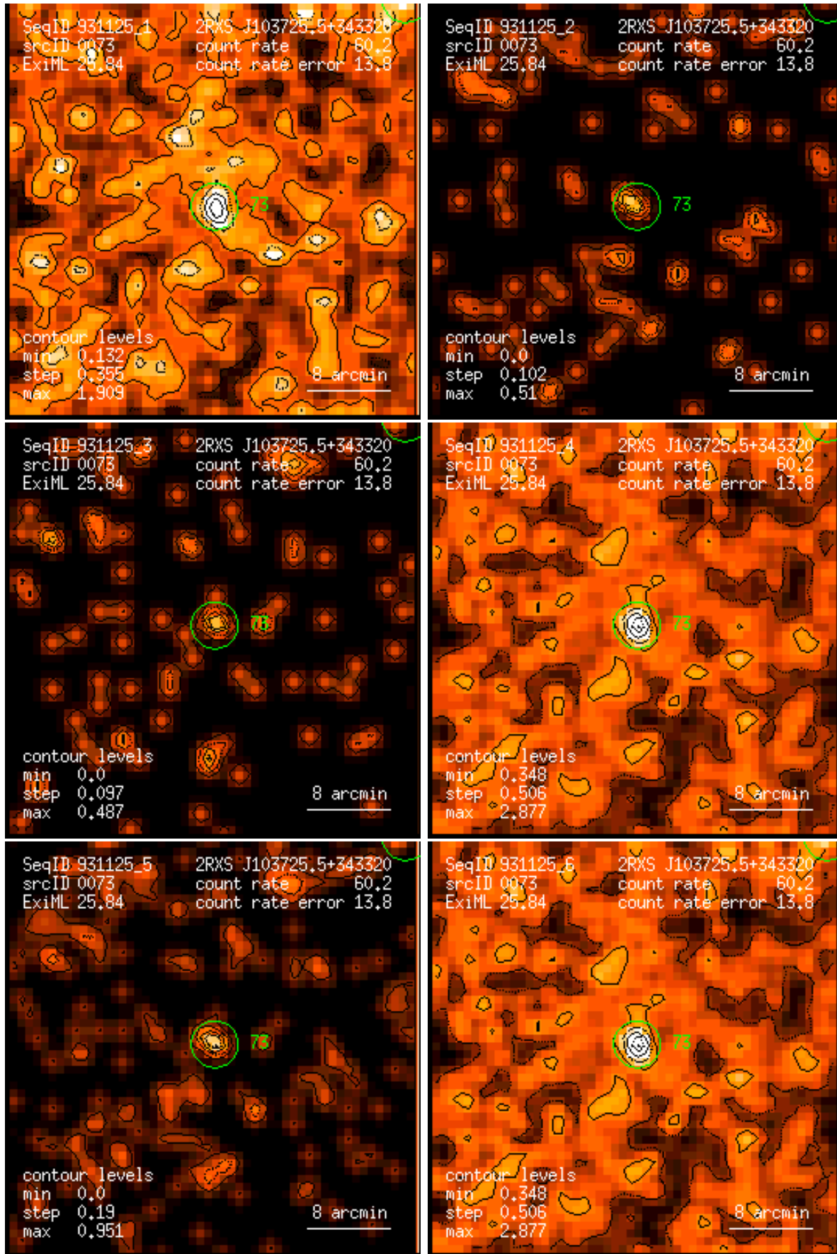
Figure 73: RASS 931125: detection 0073: band rate images, Gaussian filter: (1) PSPC channels 11 – 41, (2) 52 – 90, (3) 91 – 201, (4) 11 – 235, (5) 52 – 201, (6) 11 – 201. Broad band rates in counts/ks. Band rate contour levels in counts/ks/arcmin 2 .
