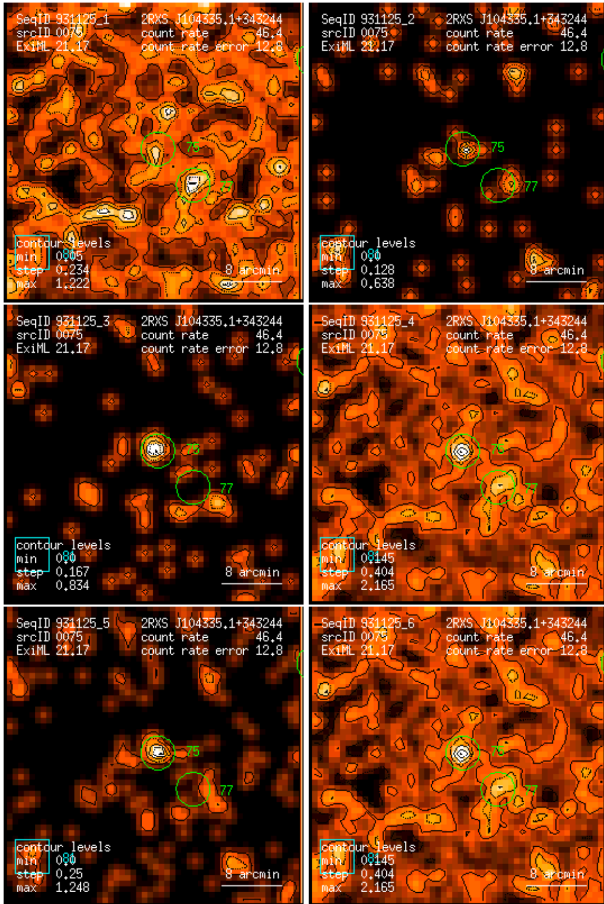
Figure 75: RASS 931125: detection 0075: band rate images, Gaussian filter: (1) PSPC channels 11 – 41, (2) 52 – 90, (3) 91 – 201, (4) 11 – 235, (5) 52 – 201, (6) 11 – 201. Broad band rates in counts/ks. Band rate contour levels in counts/ks/arcmin 2 .
