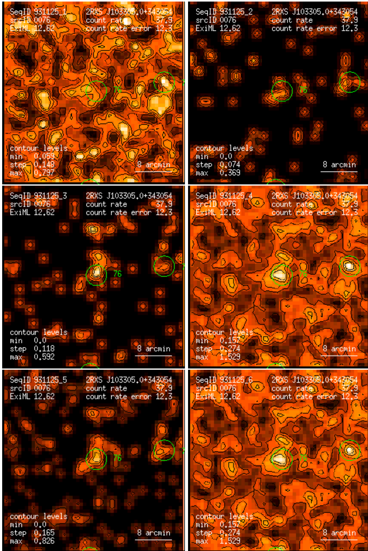
Figure 76: RASS 931125: detection 0076: band rate images, Gaussian filter: (1) PSPC channels 11 – 41, (2) 52 – 90, (3) 91 – 201, (4) 11 – 235, (5) 52 – 201, (6) 11 – 201. Broad band rates in counts/ks. Band rate contour levels in counts/ks/arcmin 2 .
