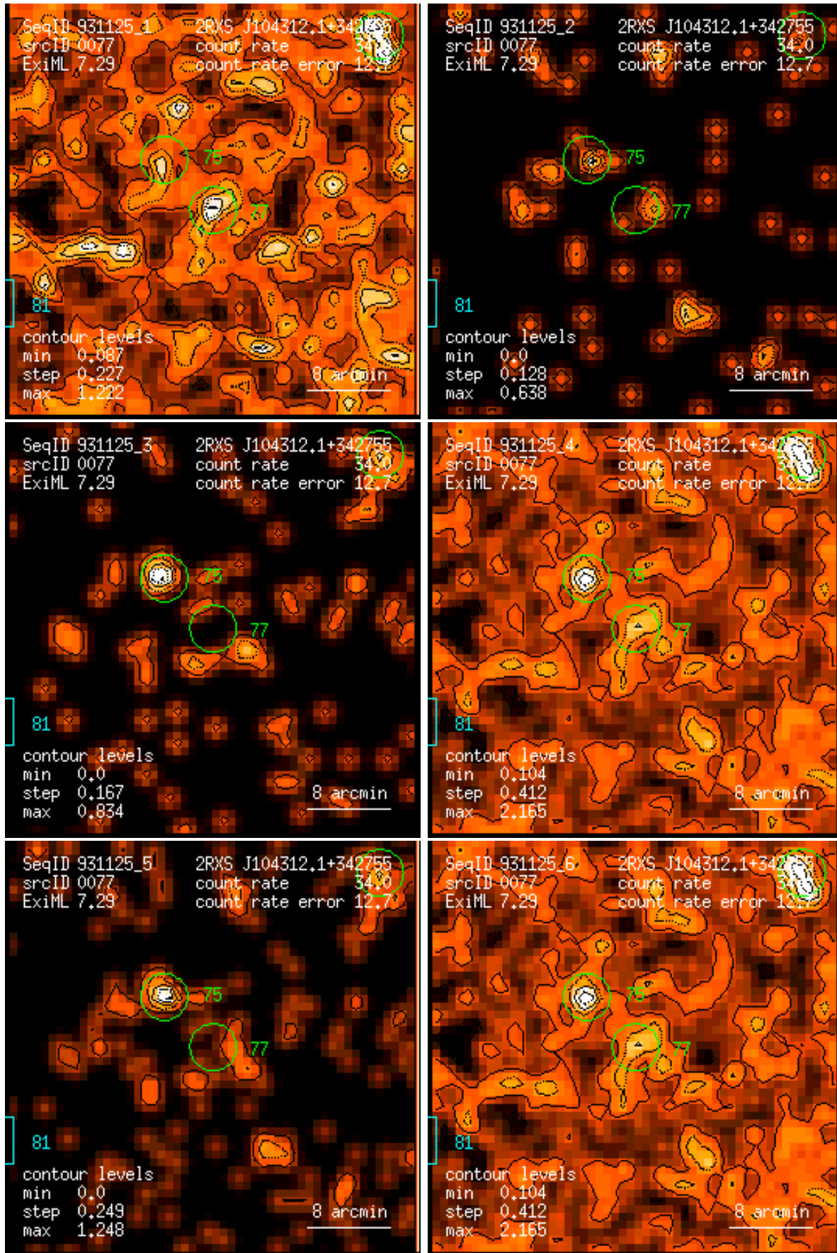
Figure 77: RASS 931125: detection 0077: band rate images, Gaussian filter: (1) PSPC channels 11 – 41, (2) 52 – 90, (3) 91 – 201, (4) 11 – 235, (5) 52 – 201, (6) 11 – 201. Broad band rates in counts/ks. Band rate contour levels in counts/ks/arcmin 2 .
