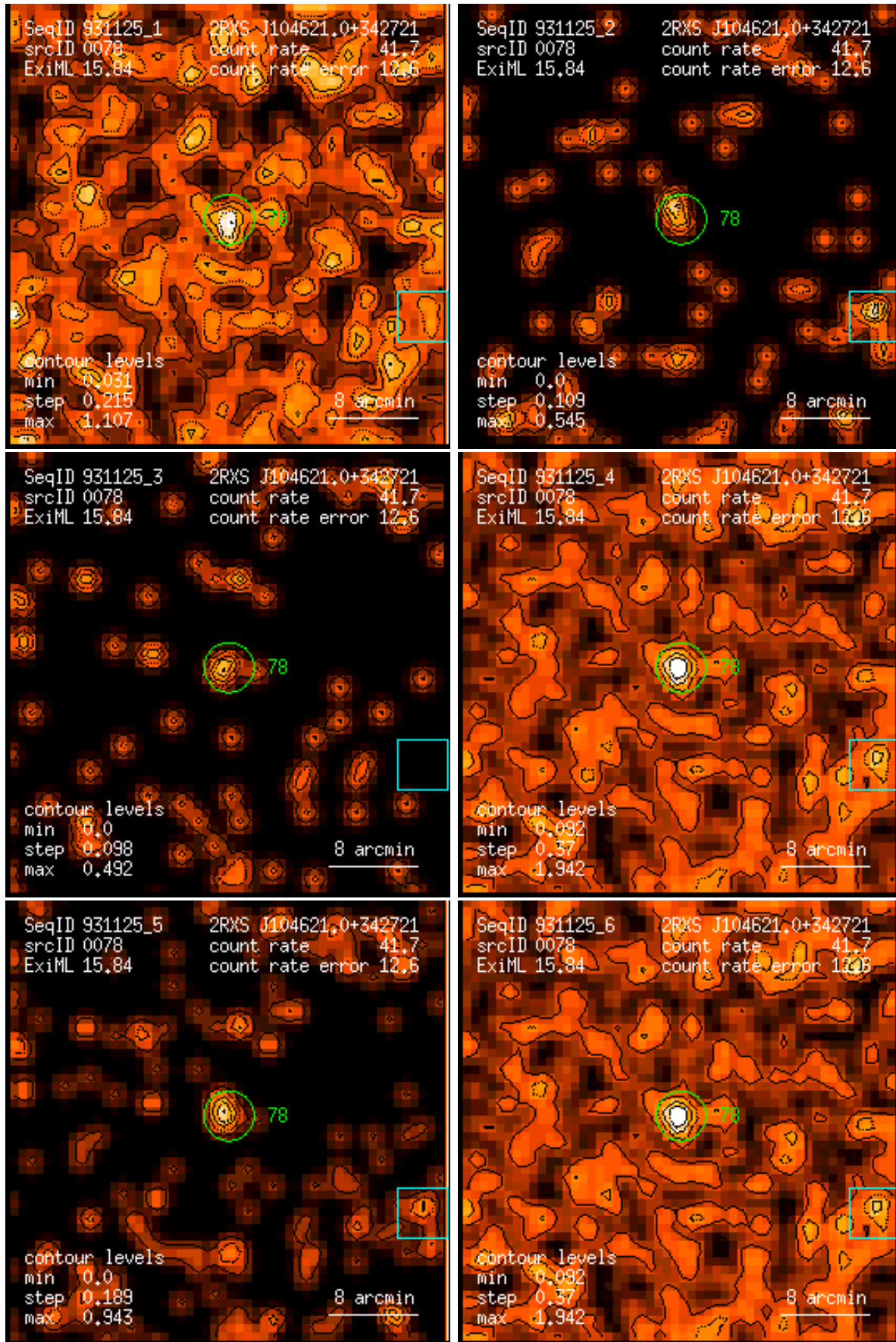
Figure 78: RASS 931125: detection 0078: band rate images, Gaussian filter: (1) PSPC channels 11 – 41, (2) 52 – 90, (3) 91 – 201, (4) 11 – 235, (5) 52 – 201, (6) 11 – 201. Broad band rates in counts/ks. Band rate contour levels in counts/ks/arcmin 2 .
