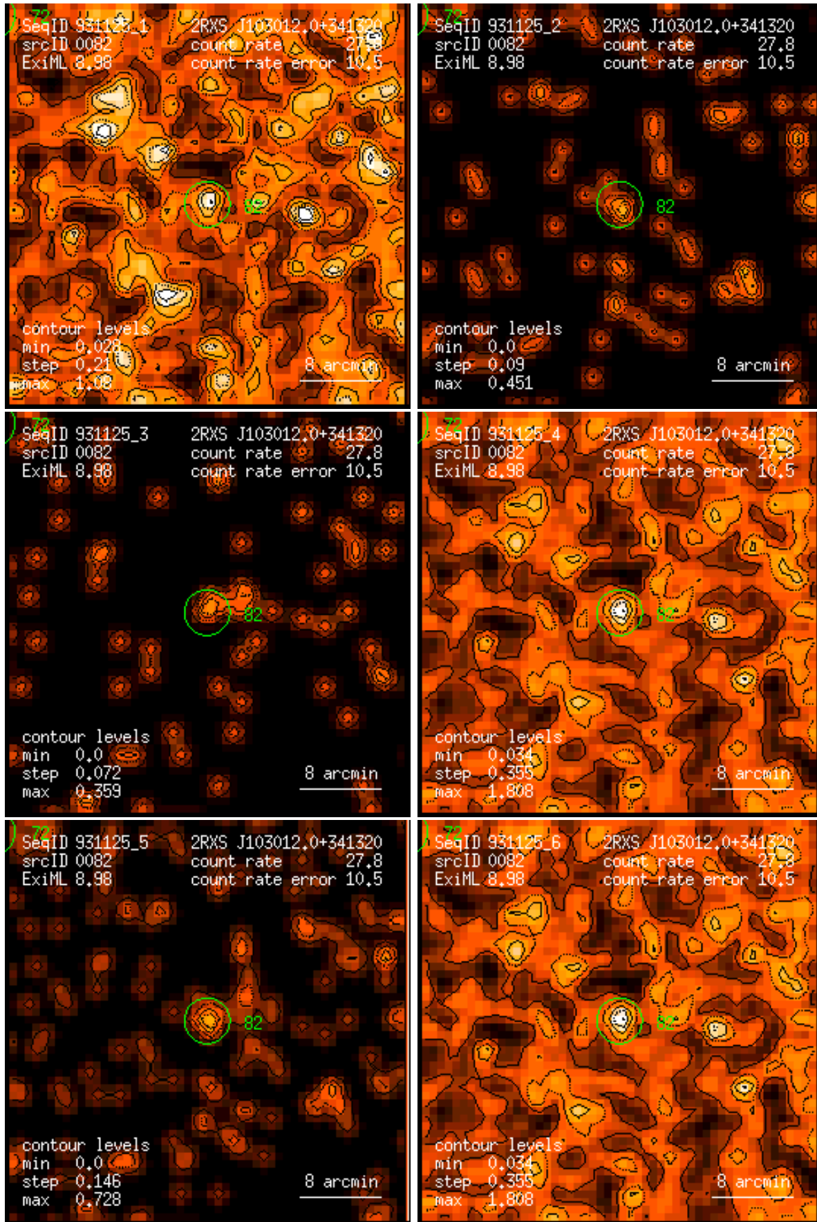
Figure 82: RASS 931125: detection 0082: band rate images, Gaussian filter: (1) PSPC channels 11 – 41, (2) 52 – 90, (3) 91 – 201, (4) 11 – 235, (5) 52 – 201, (6) 11 – 201. Broad band rates in counts/ks. Band rate contour levels in counts/ks/arcmin 2 .
