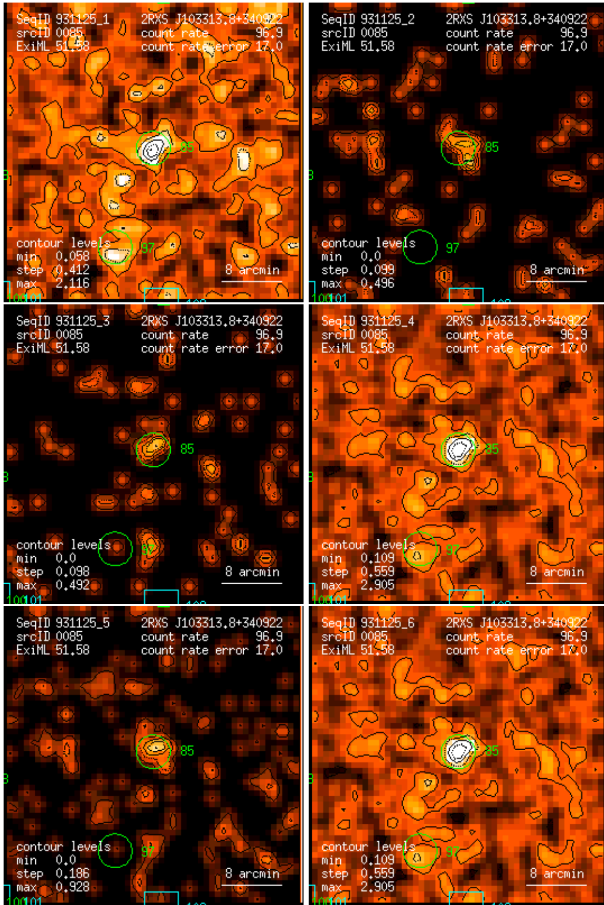
Figure 85: RASS 931125: detection 0085: band rate images, Gaussian filter: (1) PSPC channels 11 – 41, (2) 52 – 90, (3) 91 – 201, (4) 11 – 235, (5) 52 – 201, (6) 11 – 201. Broad band rates in counts/ks. Band rate contour levels in counts/ks/arcmin 2 .
