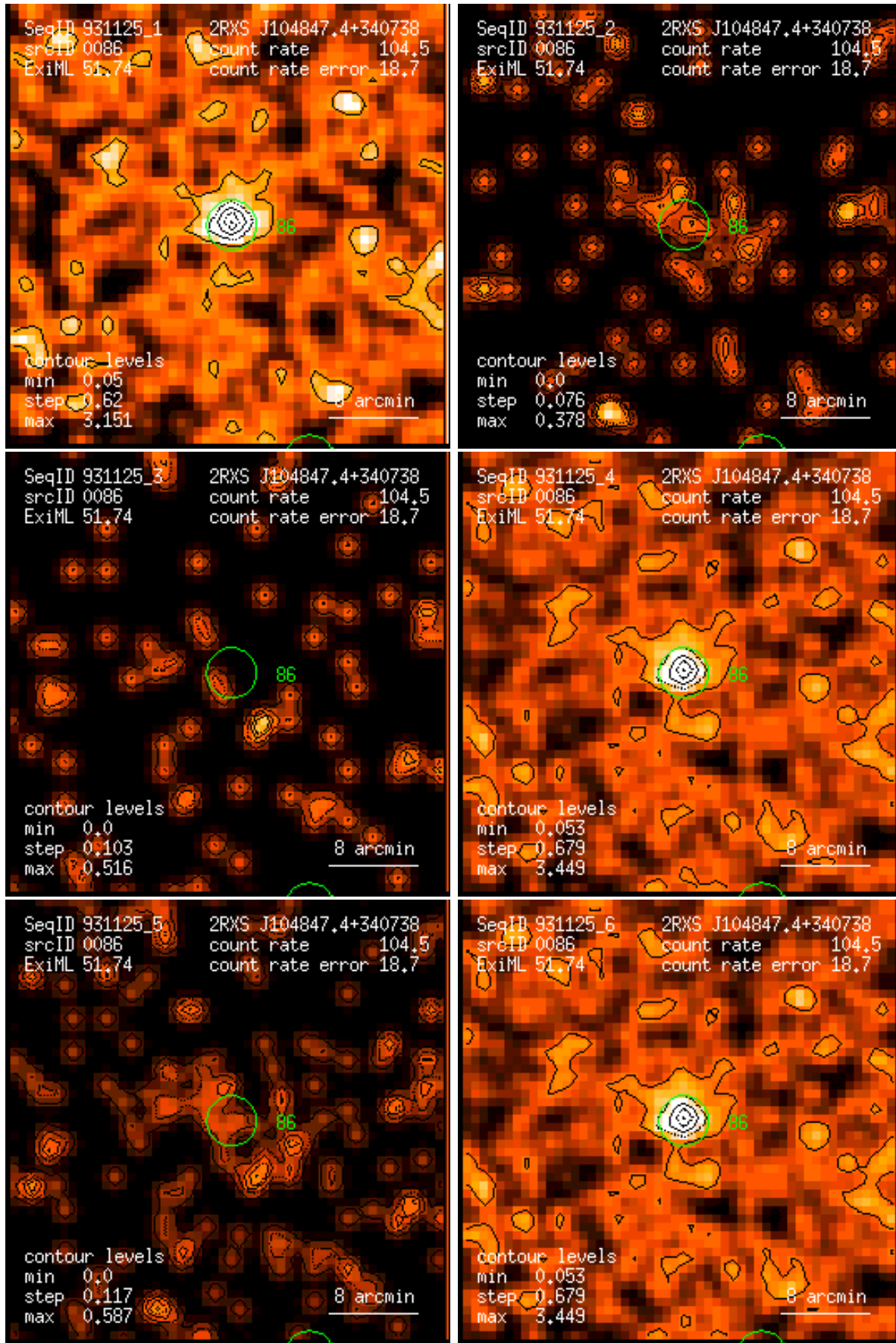
Figure 86: RASS 931125: detection 0086: band rate images, Gaussian filter: (1) PSPC channels 11 – 41, (2) 52 – 90, (3) 91 – 201, (4) 11 – 235, (5) 52 – 201, (6) 11 – 201. Broad band rates in counts/ks. Band rate contour levels in counts/ks/arcmin 2 .
