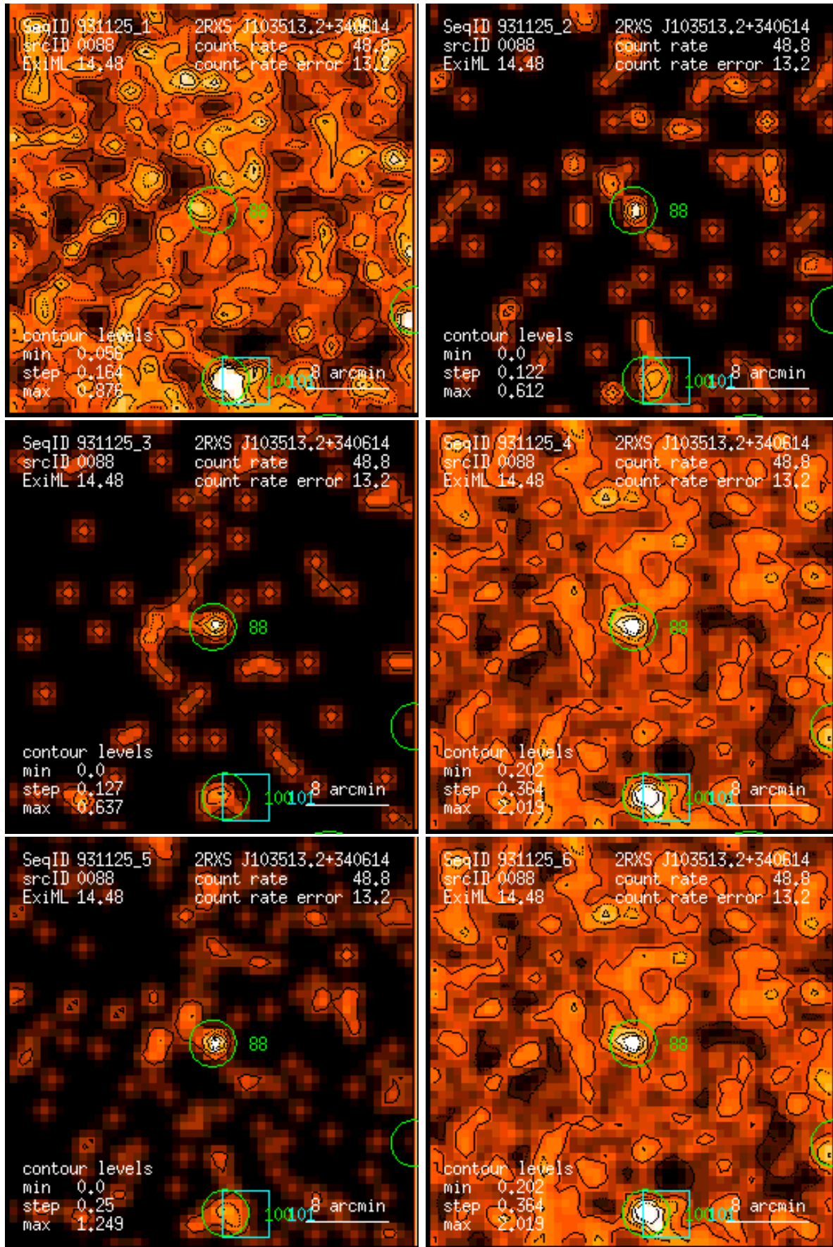
Figure 88: RASS 931125: detection 0088: band rate images, Gaussian filter: (1) PSPC channels 11 – 41, (2) 52 – 90, (3) 91 – 201, (4) 11 – 235, (5) 52 – 201, (6) 11 – 201. Broad band rates in counts/ks. Band rate contour levels in counts/ks/arcmin 2 .
