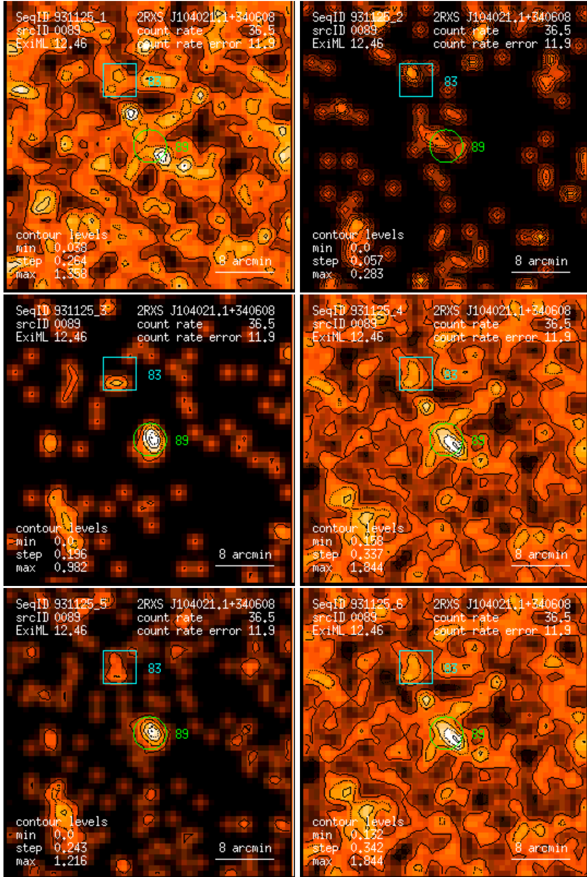
Figure 89: RASS 931125: detection 0089: band rate images, Gaussian filter: (1) PSPC channels 11 – 41, (2) 52 – 90, (3) 91 – 201, (4) 11 – 235, (5) 52 – 201, (6) 11 – 201. Broad band rates in counts/ks. Band rate contour levels in counts/ks/arcmin 2 .
