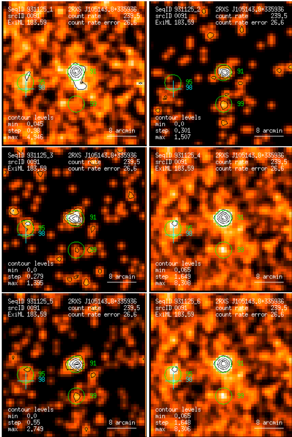
Figure 91: RASS 931125: detection 0091: band rate images, Gaussian filter: (1) PSPC channels 11 – 41, (2) 52 – 90, (3) 91 – 201, (4) 11 – 235, (5) 52 – 201, (6) 11 – 201. Broad band rates in counts/ks. Band rate contour levels in counts/ks/arcmin 2 .
