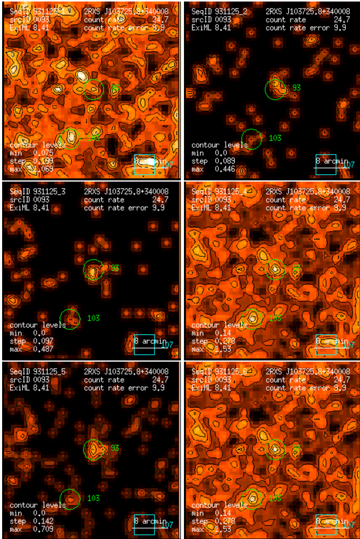
Figure 93: RASS 931125: detection 0093: band rate images, Gaussian filter: (1) PSPC channels 11 – 41, (2) 52 – 90, (3) 91 – 201, (4) 11 – 235, (5) 52 – 201, (6) 11 – 201. Broad band rates in counts/ks. Band rate contour levels in counts/ks/arcmin 2 .
