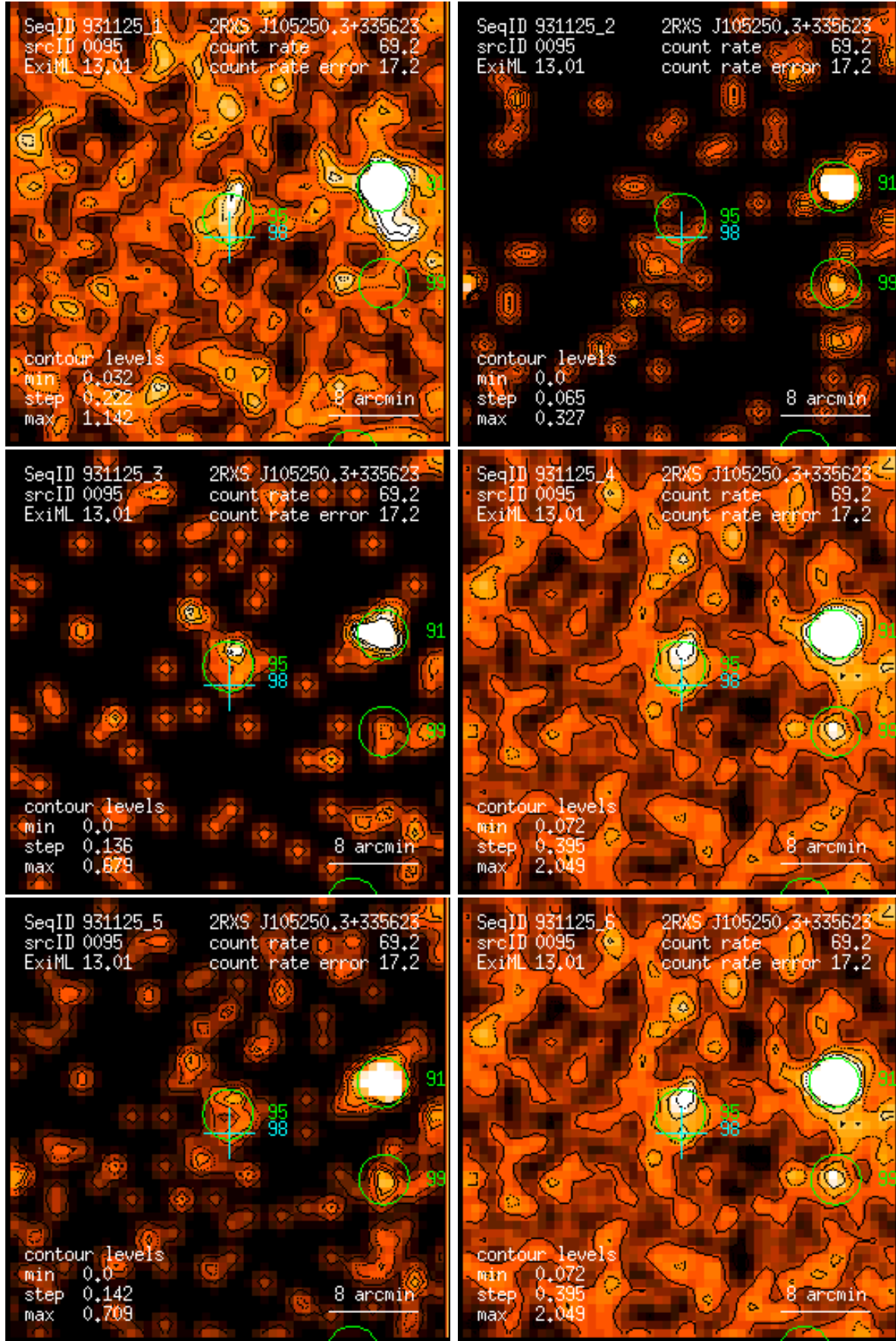
Figure 95: RASS 931125: detection 0095: band rate images, Gaussian filter: (1) PSPC channels 11 – 41, (2) 52 – 90, (3) 91 – 201, (4) 11 – 235, (5) 52 – 201, (6) 11 – 201. Broad band rates in counts/ks. Band rate contour levels in counts/ks/arcmin 2 .
